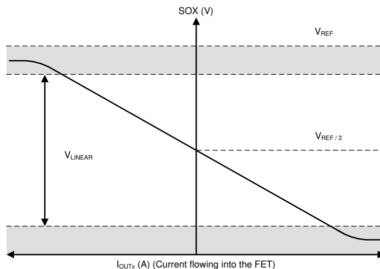
Figure 7-17. Bidirectional Current Sense Regions
