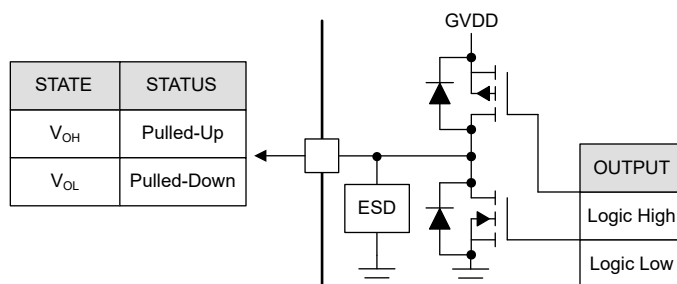
Figure 7-14. Push Pull Pin
