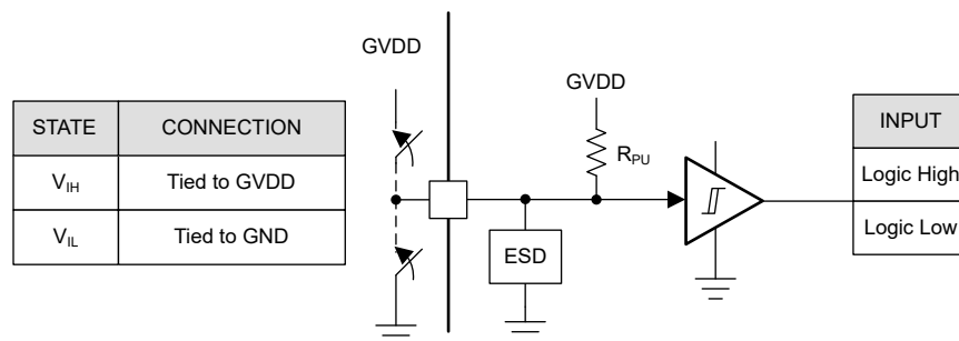
Figure 7-12. Logic nSCS
