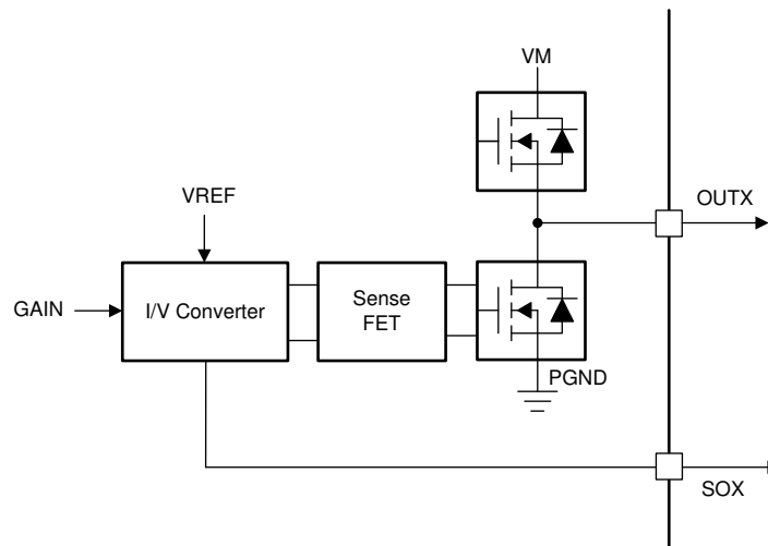
Figure 7-15. Integrated Current Sense Amplifier
