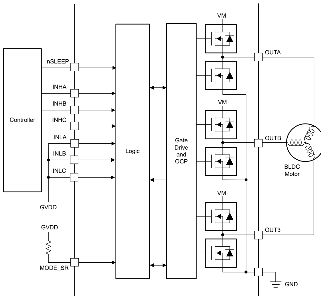
Figure 7-3. 3x PWM Mode
