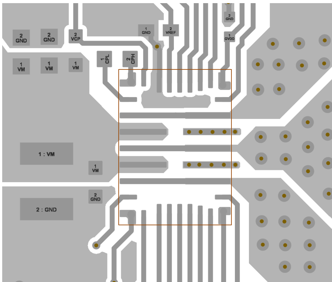
Figure 9-5. Layout example for VQFN 29 pin package
