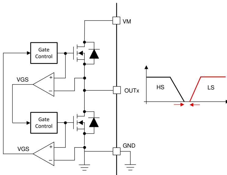
Figure 7-9. Cross Conduction Protection
