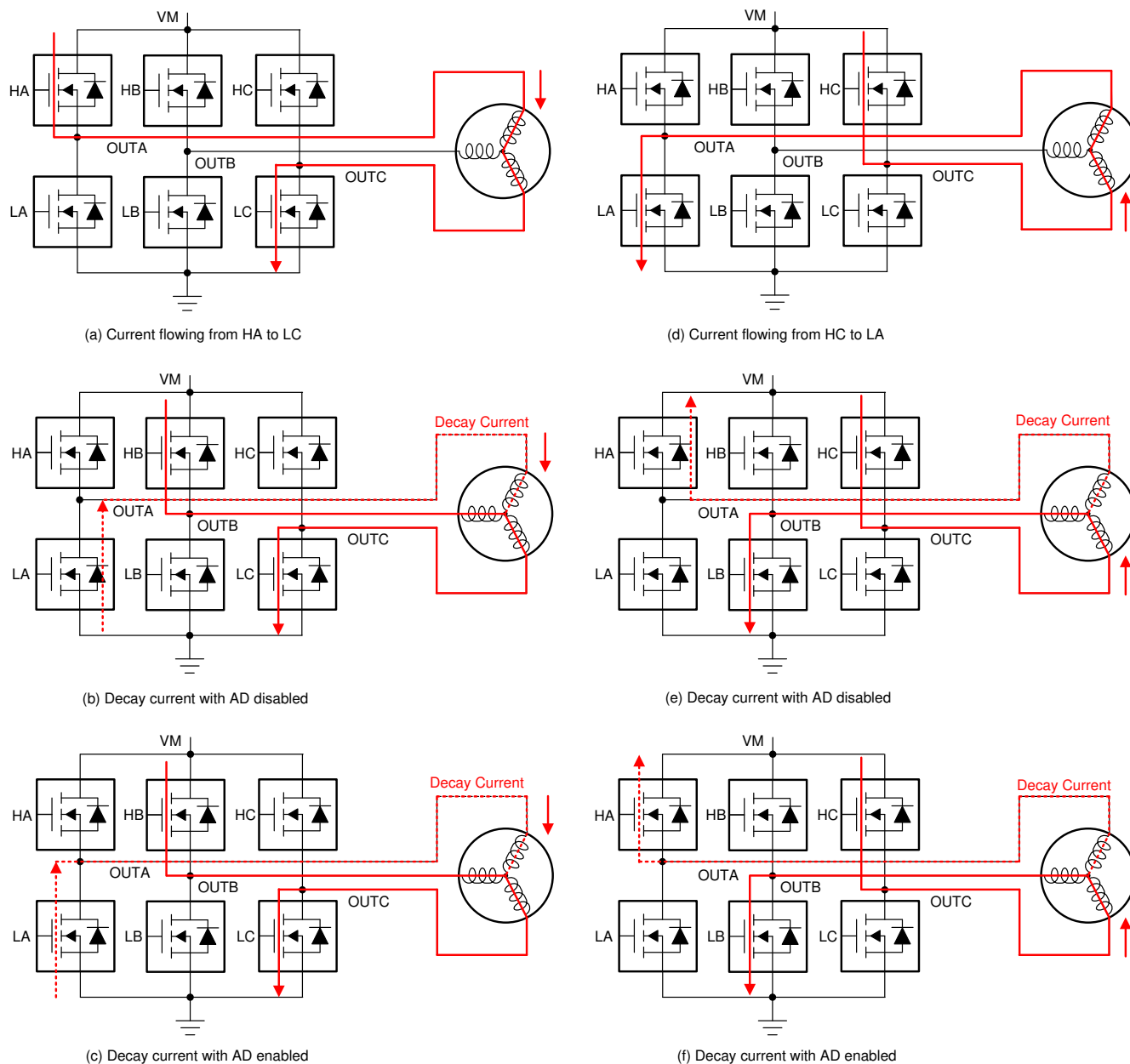
Figure 7-19. ASR in BLDC Motor Commutation
