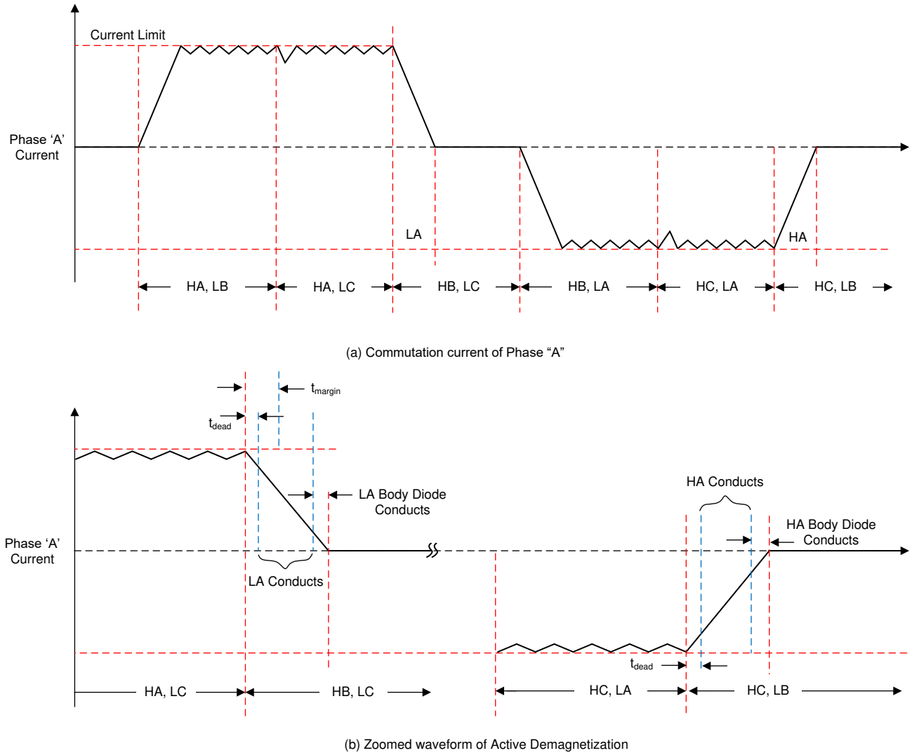
Figure 7-20. Current Waveforms for ASR in BLDC Motor Commutation
