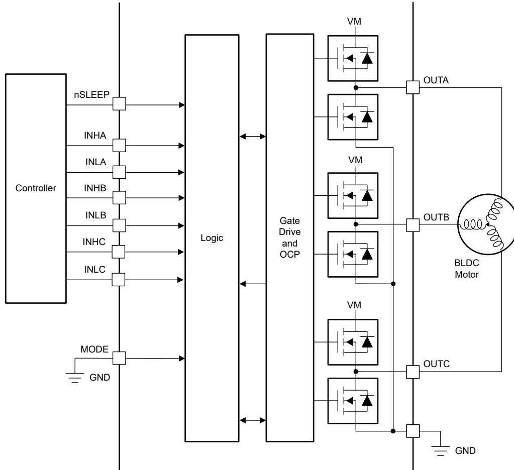
Figure 7-4. 6x PWM Mode
