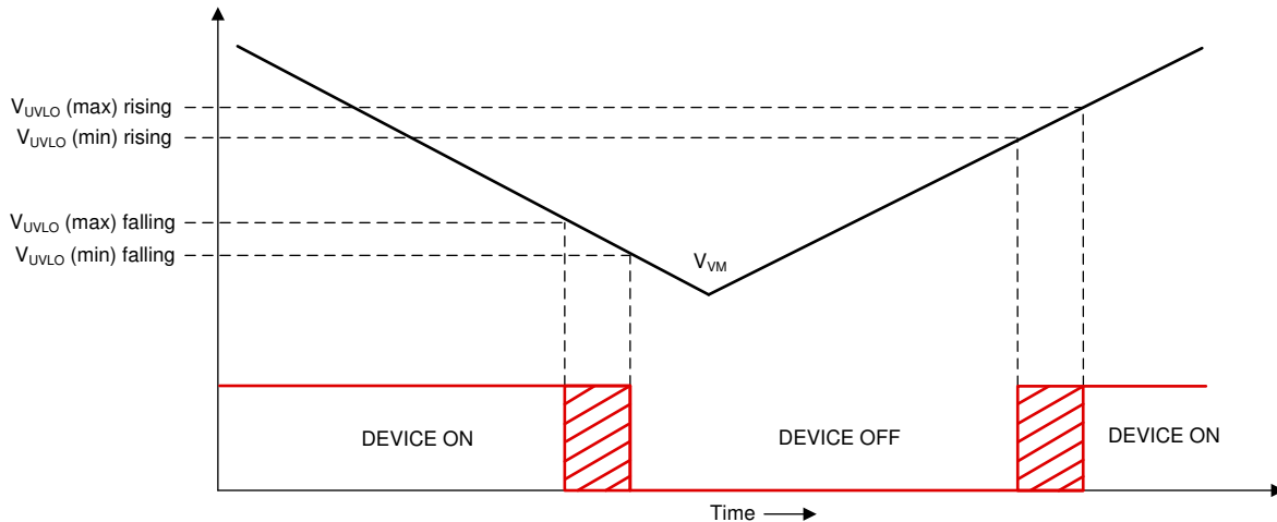
Figure 7-25. VM Supply Undervoltage Lockout
