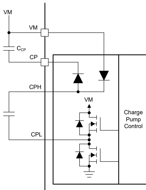
Figure 7-6. Charge Pump
