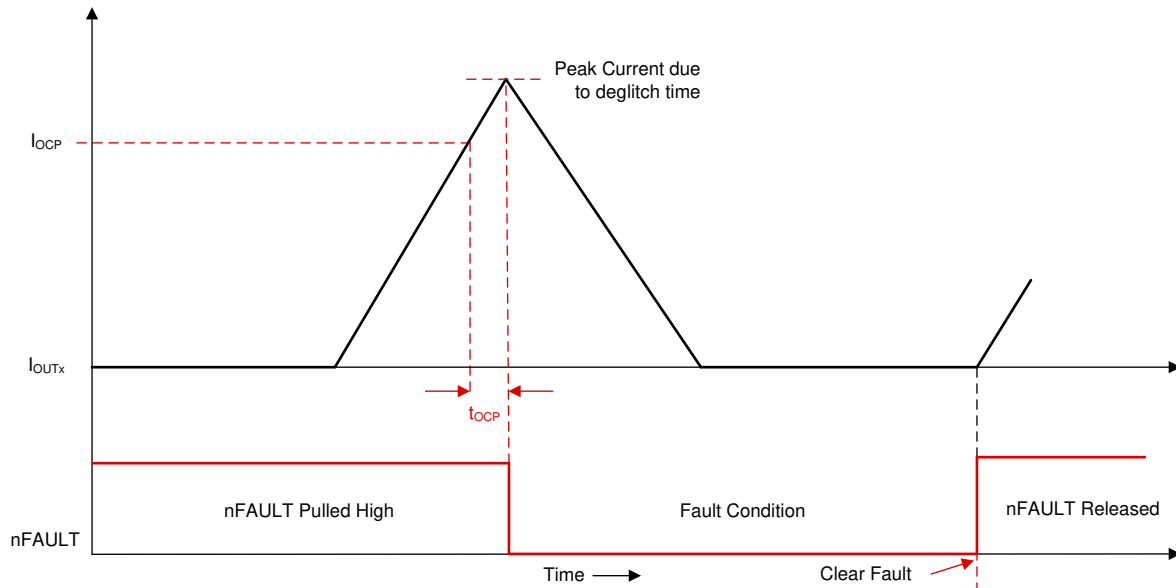
Figure 7-23. Overcurrent Protection - Latched Shutdown Mode
