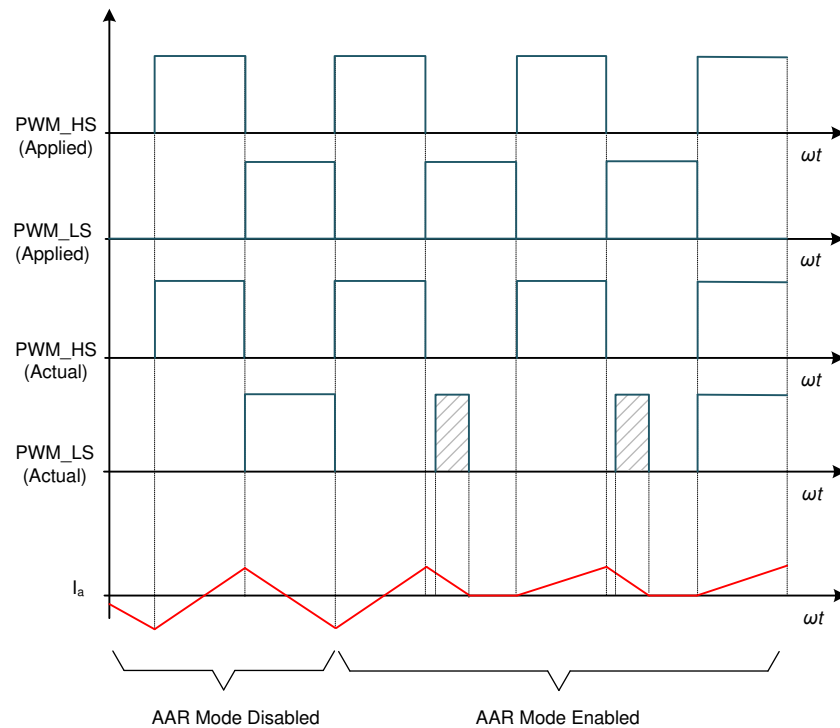
Figure 7-22. AAR in PWM Mode
