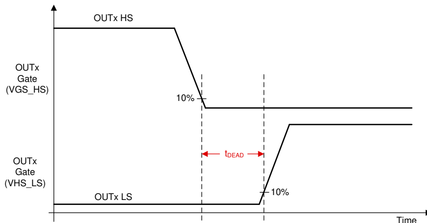
Figure 7-10. Dead Time
