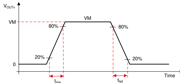
Figure 7-8. Slew Rate Timings
