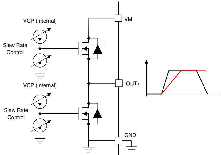
Figure 7-7. Slew Rate Circuit Implementation
