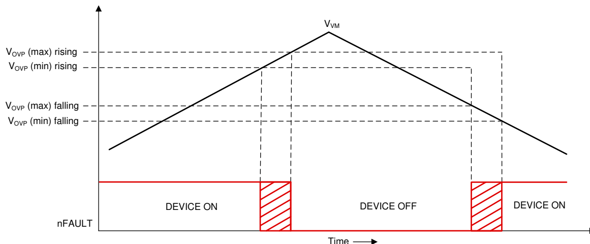
Figure 7-26. Over Voltage Protection
