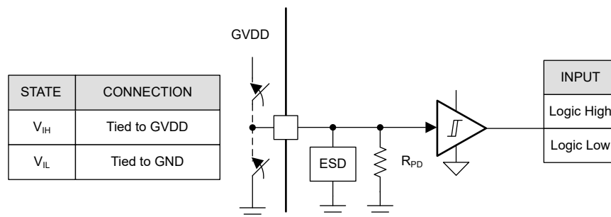
Figure 7-11. Logic-Level Input Pin Structure
