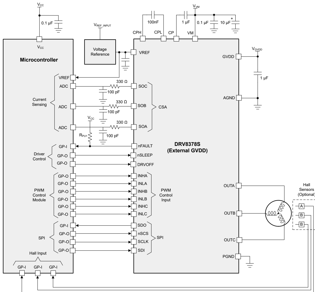
Figure 9-3. Primary Application Schematics 29pin DRV8378G SPI Variant
