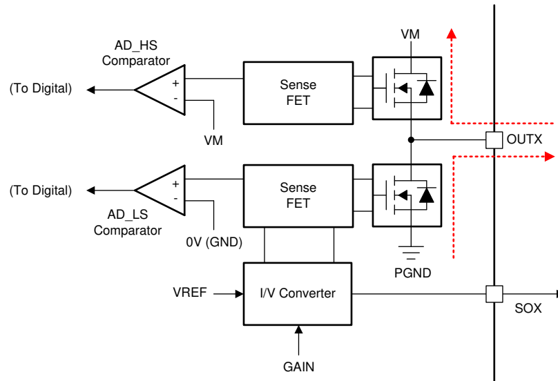
Figure 7-18. Active Demagnetization Operation
