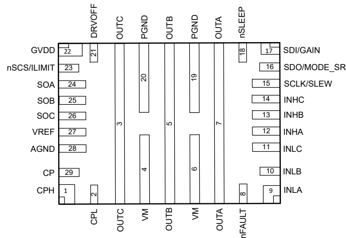
Figure 5-1. DRV8378-Q1 29-Pin VQFN Top View
