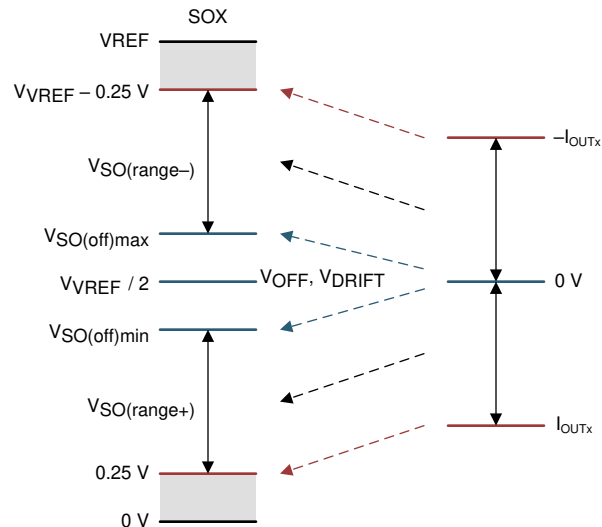
Figure 7-16. Bidirectional Current Sense Output
