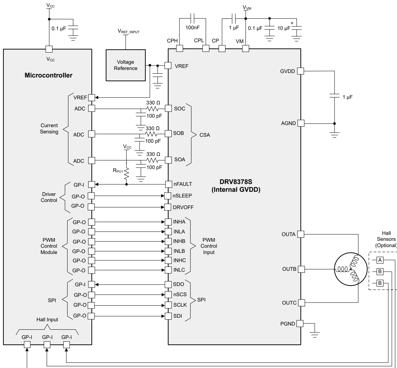
Figure 9-1. Primary Application Schematics 29pin DRV8378 SPI Variant
