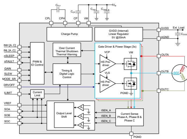
Figure 7-2. DRV8378H(29-Pin Hardware Variant) Block Diagram
