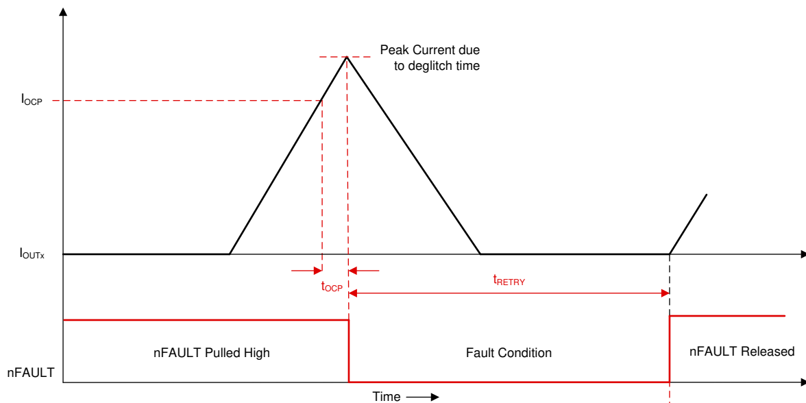
Figure 7-24. Overcurrent Protection - Automatic Retry Mode
