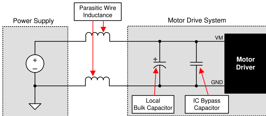
Figure 9-23. Example Setup of Motor Drive System With External Power Supply
