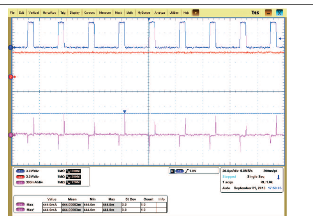
Figure 13. Output Pulse Width Modulating at VCC = 5 V
