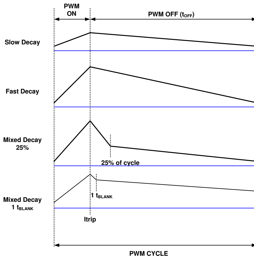
Figure 8. Decay Behavior
