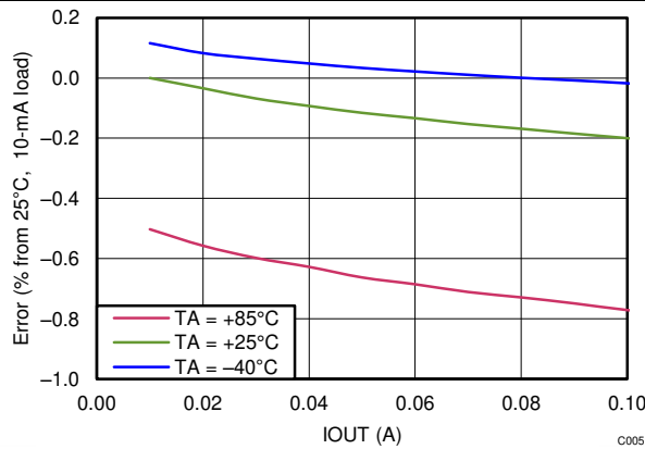
Figure 9. LDO Output, V CC = 3.5 V, LDOOUT = 3.3 V
