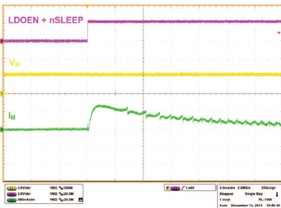
Figure 19. I_M Start-Up after LDOEN and nSLEEP Toggle
