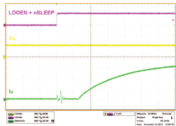
Figure 20. I_M Start-Up Delay after LDOEN and nSLEEP Toggle
