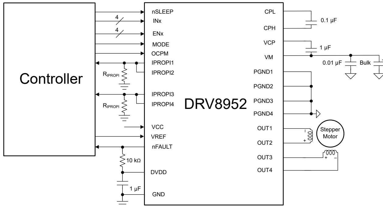
Figure 7-4. Driving Stepper Motor with DRV8952
