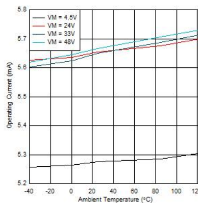
Figure 6-4. Operating Current over Temperature
