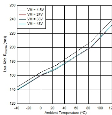
Figure 6-6. Low-Side R_{DS(ON)} over Temperature (MODE = 0 or 330k to GND)
