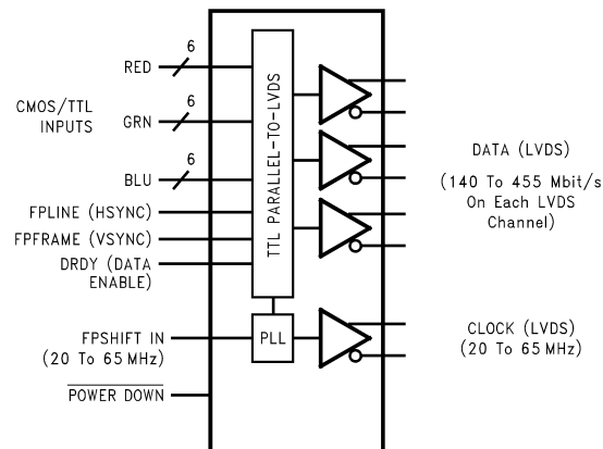
Figure 1. DS90C363B
