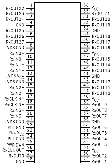
DS90CF384MTD
