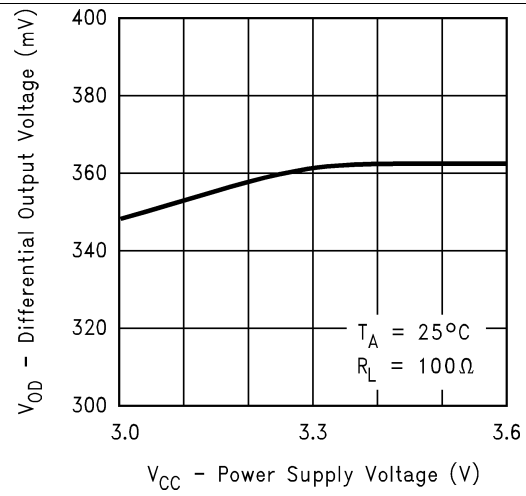
Figure 4. Differential Output Voltage vs Power Supply Voltage
