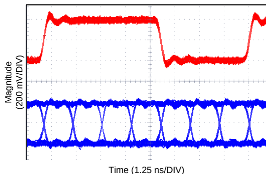
Figure 39. 96 MHz TxCLKOUT± and TxOUT0± Data Output
