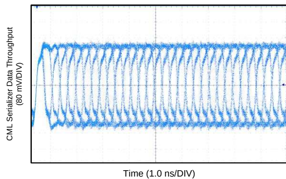
Figure 17. Serializer Output Stream with 96 MHz Input Clock
