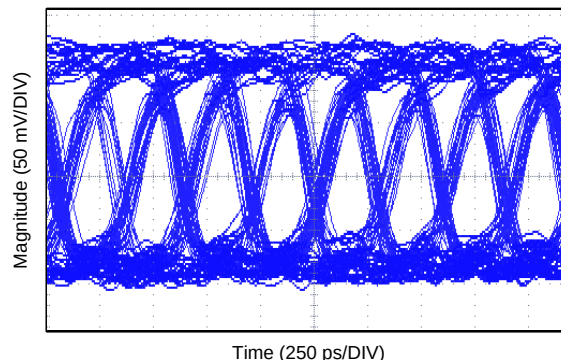
Figure 40. CMLOUT of Deserializer from 96 MHz Input Clock
