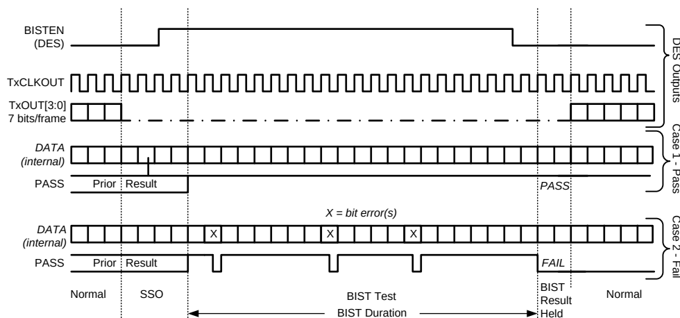
Figure 21. BIST Waveforms
