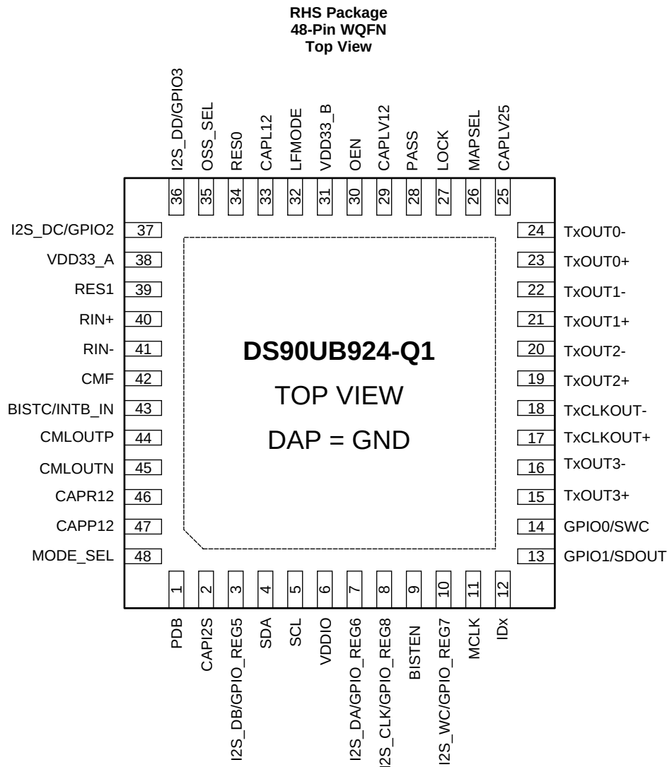
Pin Functions
