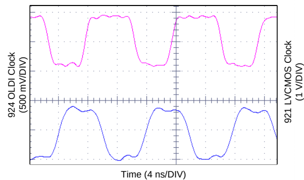
Figure 18. 96 MHz Clock at Serializer and Deserializer
