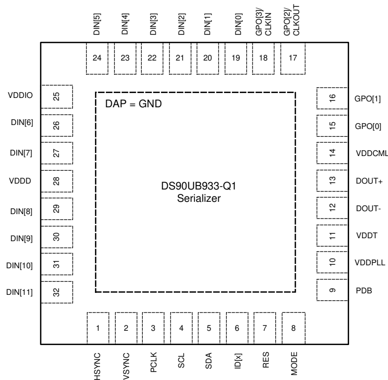
Figure 5-1. RTV Package 32-Pin WQFN Top View
