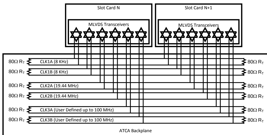
Figure 1. System Diagram
