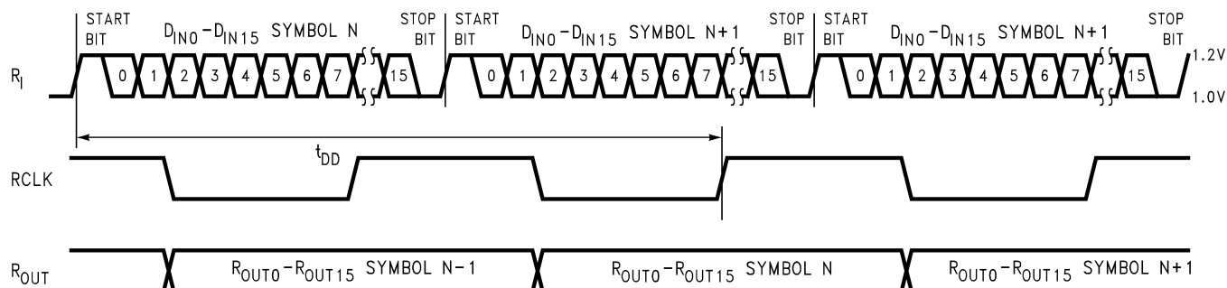
Figure 11. Deserializer Delay
