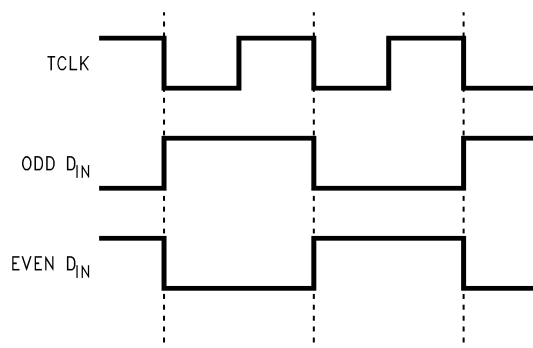
Figure 2. "Worst Case" Serializer ICC Test Pattern
