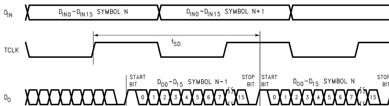
Figure 10. Serializer Delay
