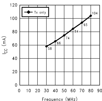
Figure 21. I_{\text{CC}} vs Freq (Tx only)
