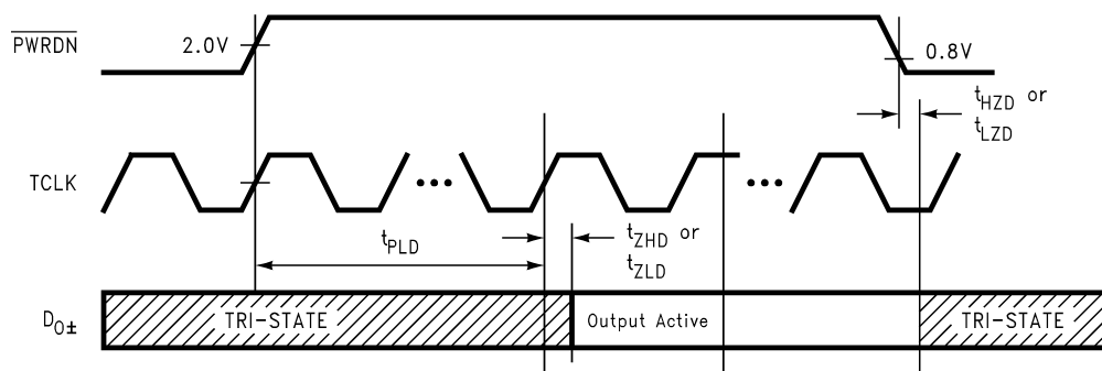
Figure 9. Serializer PLL Lock Time, SYNC Timing and \overline{\text{PWRDN}} TRI-STATE Delays
