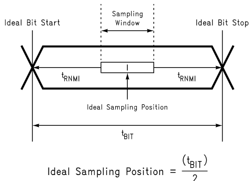
Figure 17. Deserializer Noise Margin ( t_{\text{RNMI}} ) and Sampling window
