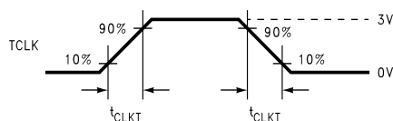
Figure 6. Serializer Input Clock Transition Time
