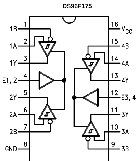
Figure 2. Top View
