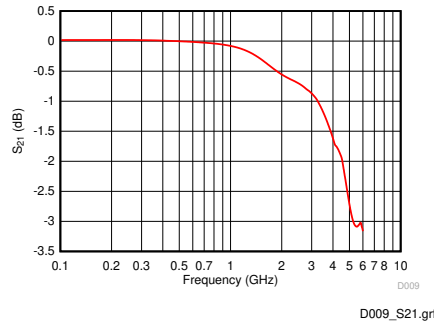
Figure 7-2. Insertion Loss Vs. Frequency
