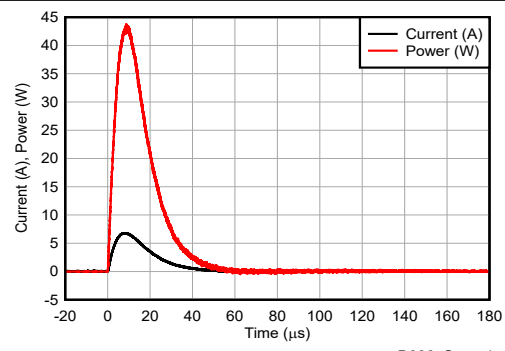
Figure 5-6. Surge Curve (IEC 61000-4-5, t_p=8/20\mu\text{s} ), I/O Pin to GND
