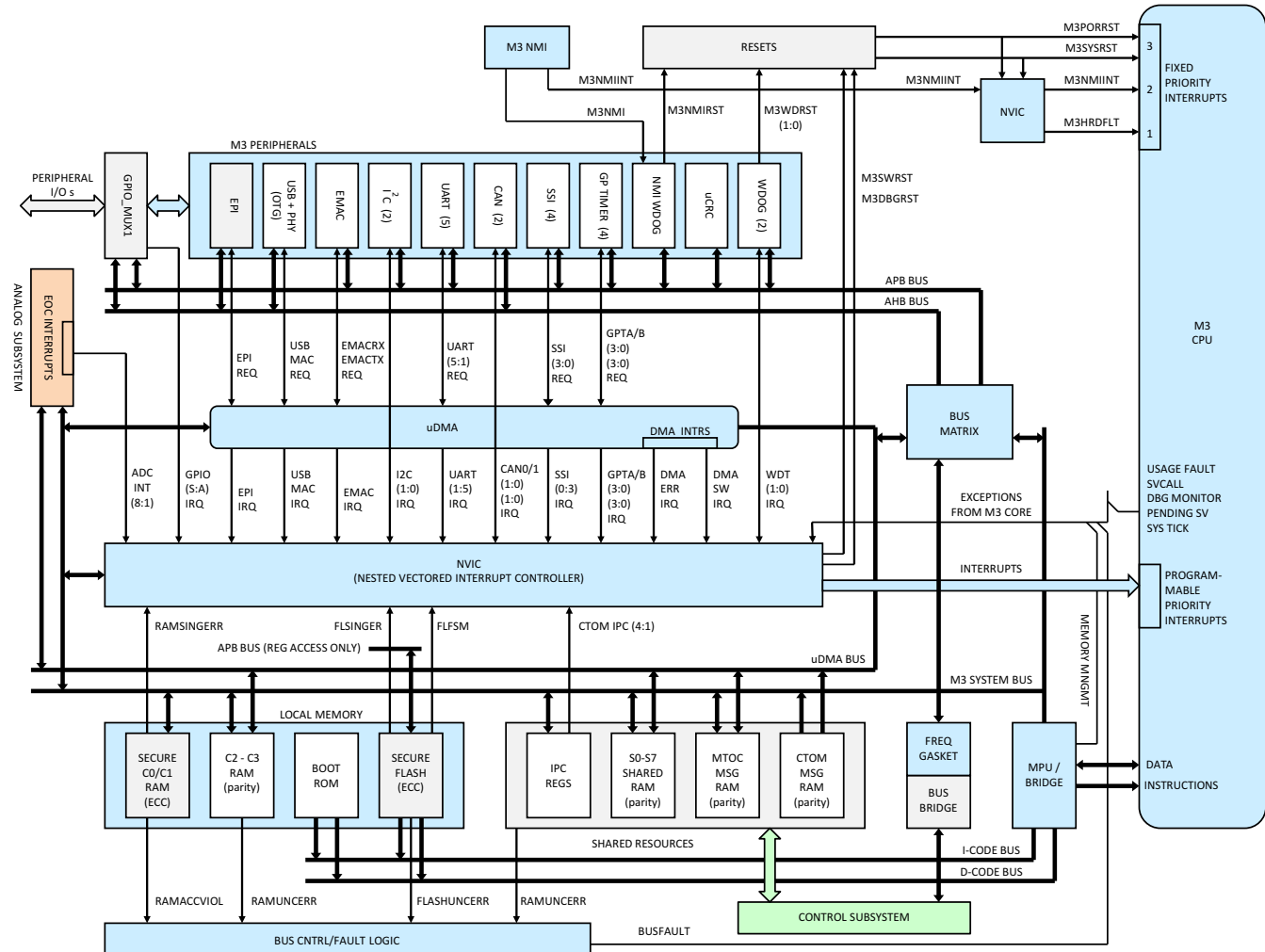
Figure 8-1. Master Subsystem
