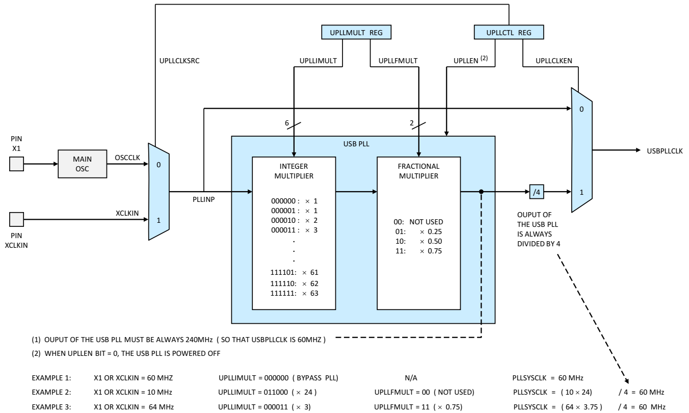
Figure 8-9. USB PLL
