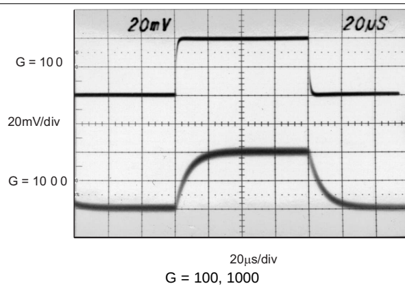
Figure 24. Small Signal
