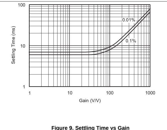
Figure 9. Settling Time vs Gain
