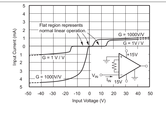
Figure 11. Input Overvoltage Voltage-to-Current Characteristics
