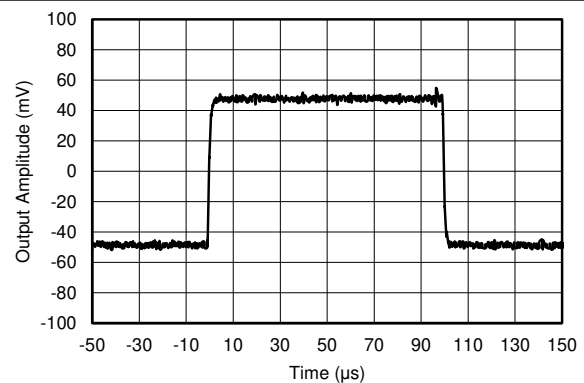
Figure 6-32. Small Signal
