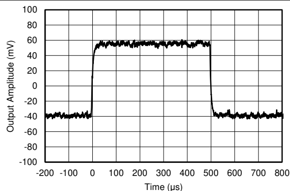
Figure 6-33. Small Signal
