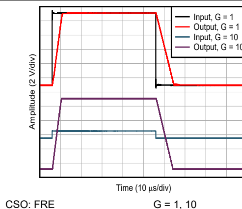
Figure 6-38. Large Signal
