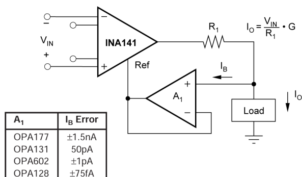
Figure 6-8. Differential Voltage-to-Current Converter
