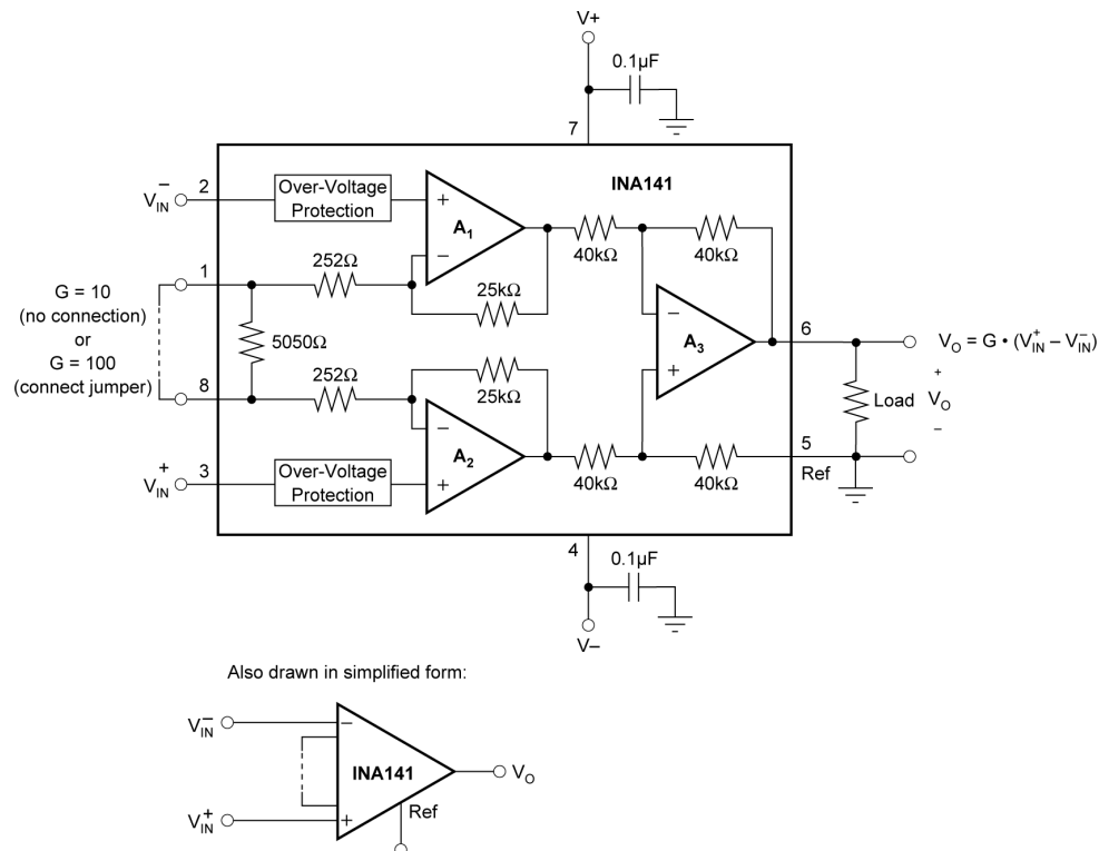
Figure 6-1. Basic Connections.
