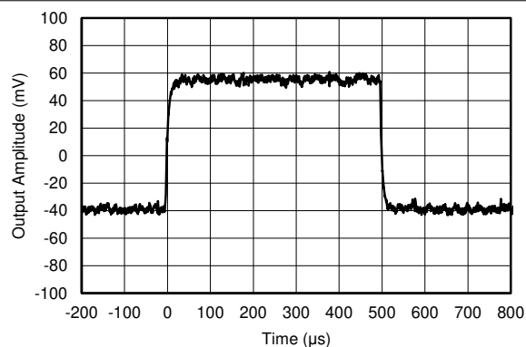
Figure 5-33. Small-Signal Step Response
