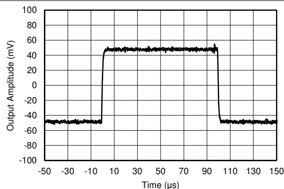
Figure 5-32. Small-Signal Step Response
