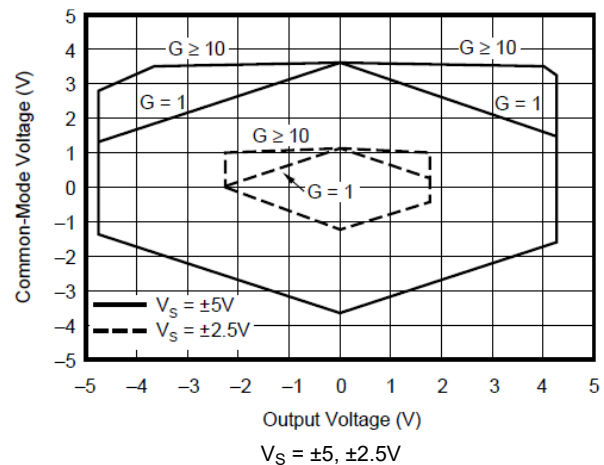
Figure 5-10. Input Common-Mode Range vs Output Voltage
