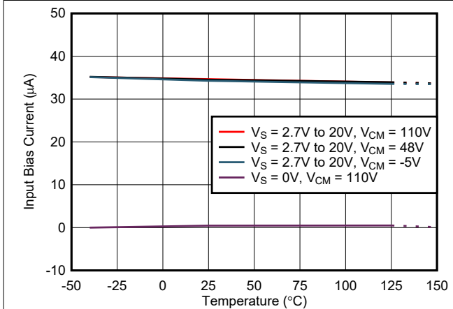
Figure 6-17. Input Bias Current vs Temperature
