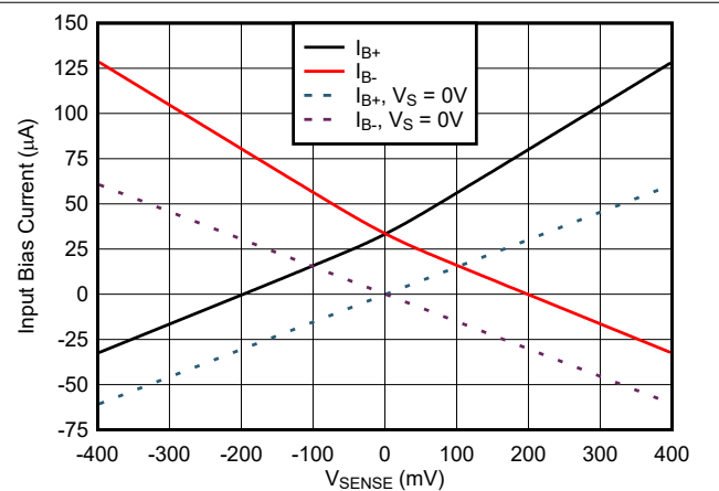
Figure 6-20. INA241x3-Q1 and INA241x4-Q1 Input Bias Current vs V_{\text{SENSE}}
