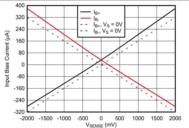
Figure 6-18. INA241x-Q1 Input Bias Current vs V_{\text{SENSE}}
