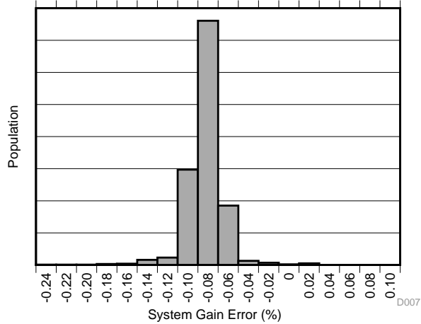
Figure 7. Gain Error Production Distribution (INA253A2)
