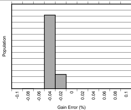
Figure 11. Gain Error Distribution (INA301A2)
