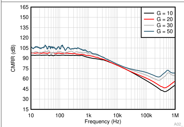
Figure 7-29. CMRR (Referred to Input) vs Frequency
