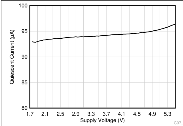
Figure 7-25. Quiescent Current vs Supply Voltage
