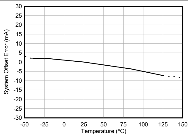
Figure 5-3. INA751A Input Offset Current vs Temperature
