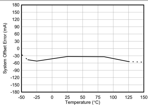
Figure 5-4. INA751B Input Offset Current vs Temperature
