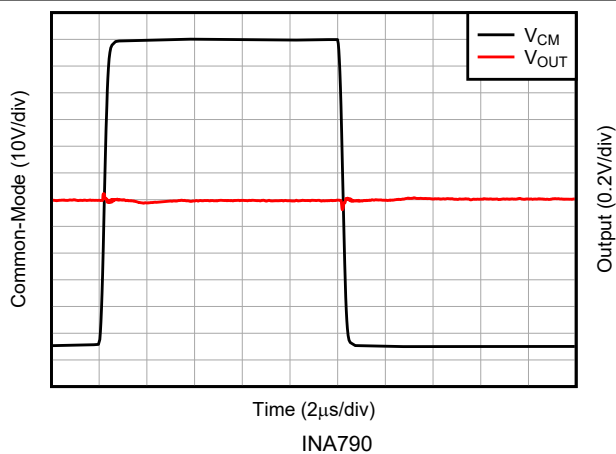
Figure 5-34. -4V to 110V Common-Mode Step Transient Response
