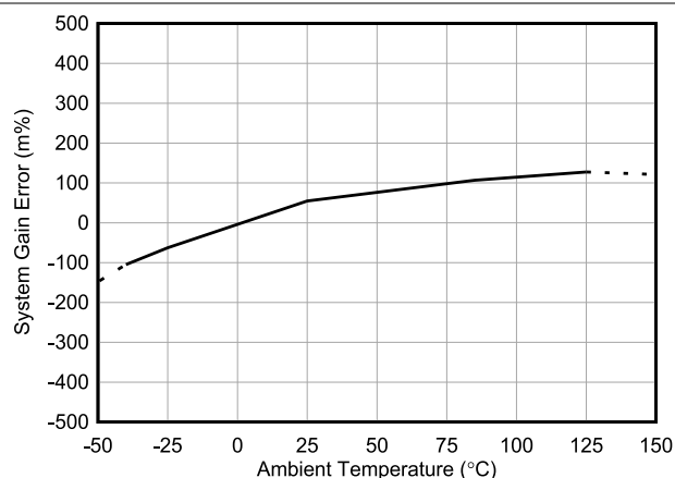
Figure 5-14. INA790B Gain Error vs Temperature
