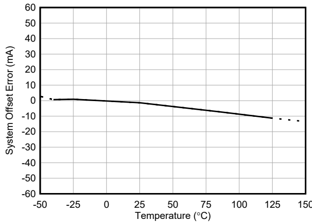
Figure 5-3. INA790A Input Offset Current vs Temperature
