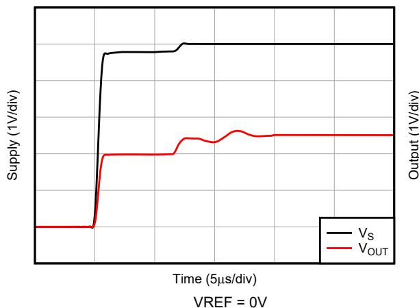
Figure 5-35. Start-Up Response
