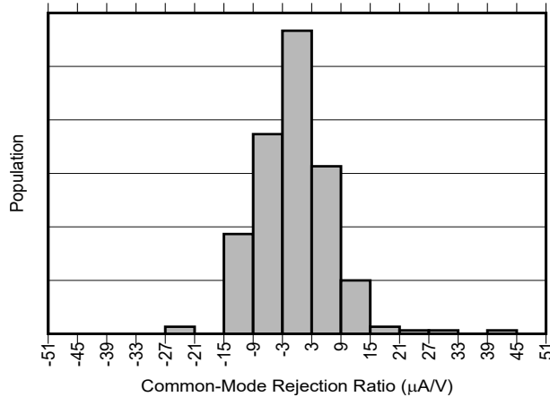
Figure 5-5. INA790A Common-Mode Rejection Production Distribution
