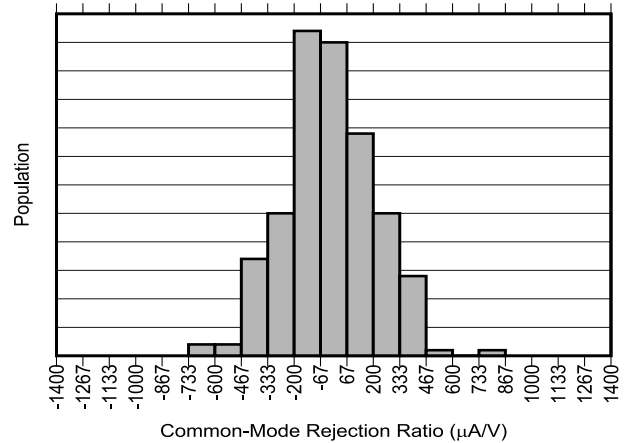
Figure 5-6. INA790B Common-Mode Rejection Production Distribution
