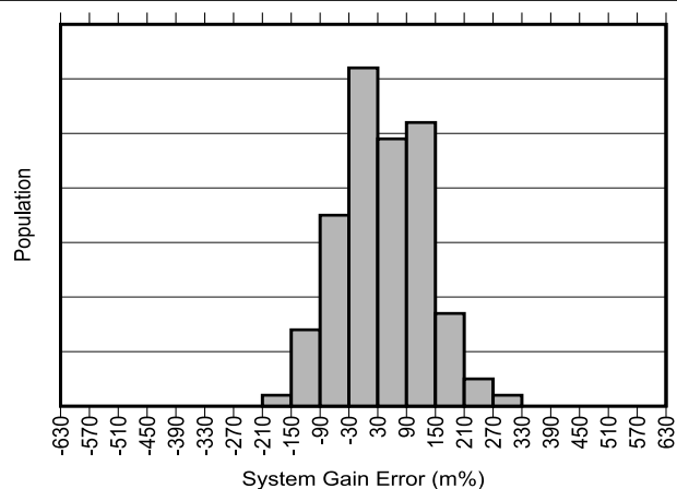
Figure 5-12. INA790B Gain Error Production Distribution
