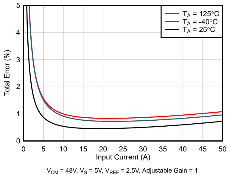
Figure 7-1. INA790A Total Error vs Input Current
