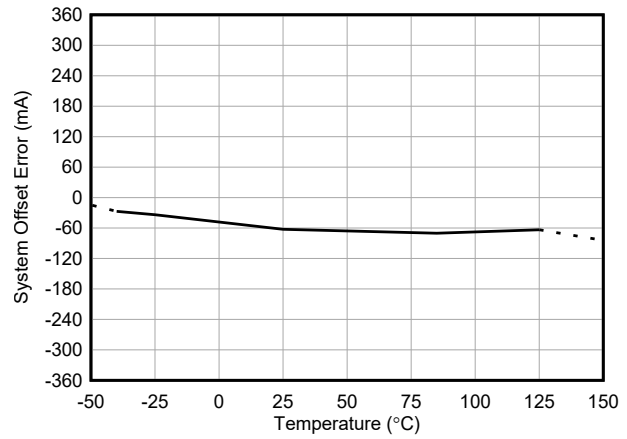
Figure 5-4. INA790B Input Offset Current vs Temperature
