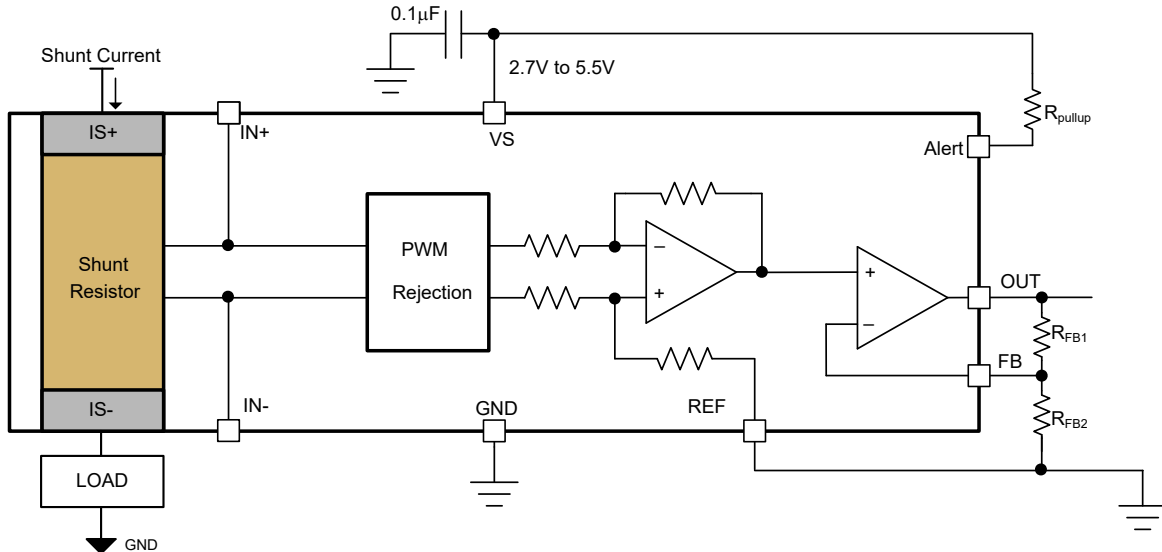
Figure 6-6. Ground-Referenced Output
