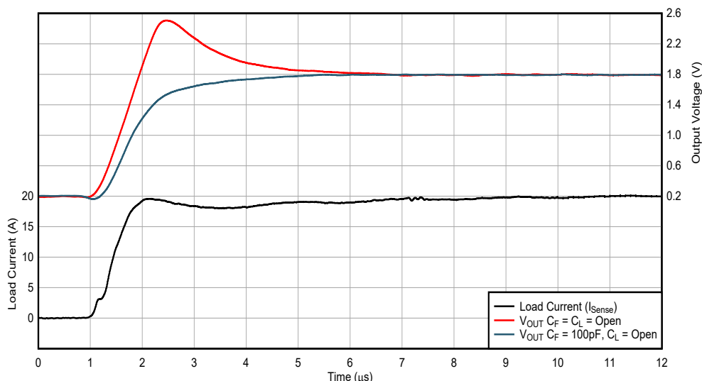
Figure 7-6. INA790x Load Step Responses Before and After RISO Dual Feedback for Adjustable Gain of 1
