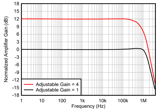
Figure 5-26. Current Sense Amplifier Gain vs Frequency
