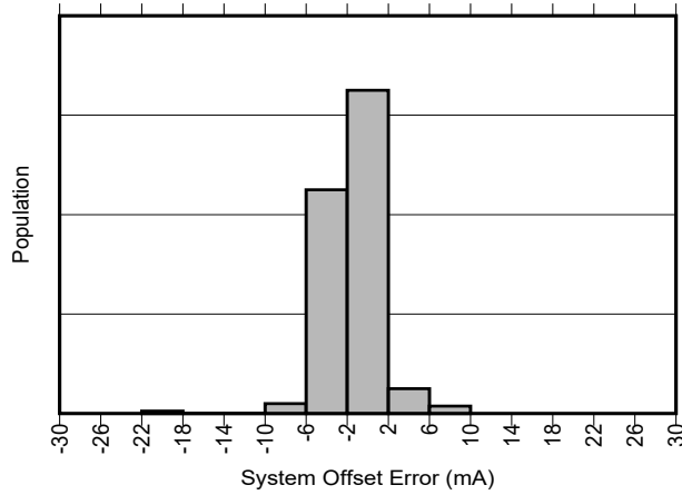
Figure 5-1. INA790A Input Offset Current Production Distribution
