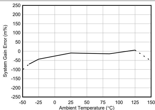
Figure 5-13. INA790A Gain Error vs Temperature
