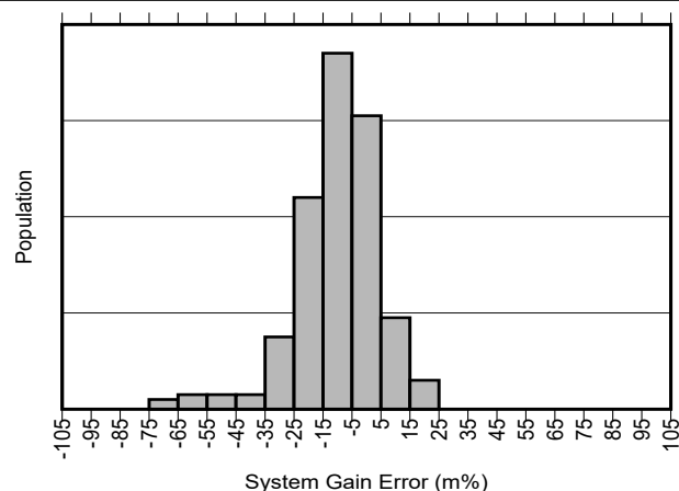
Figure 5-11. INA790A Gain Error Production Distribution
