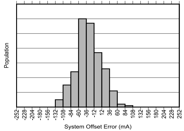
Figure 5-2. INA790B Input Offset Current Production Distribution
