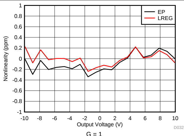
Figure 33. Gain Nonlinearity
