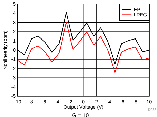
Figure 34. Gain Nonlinearity
