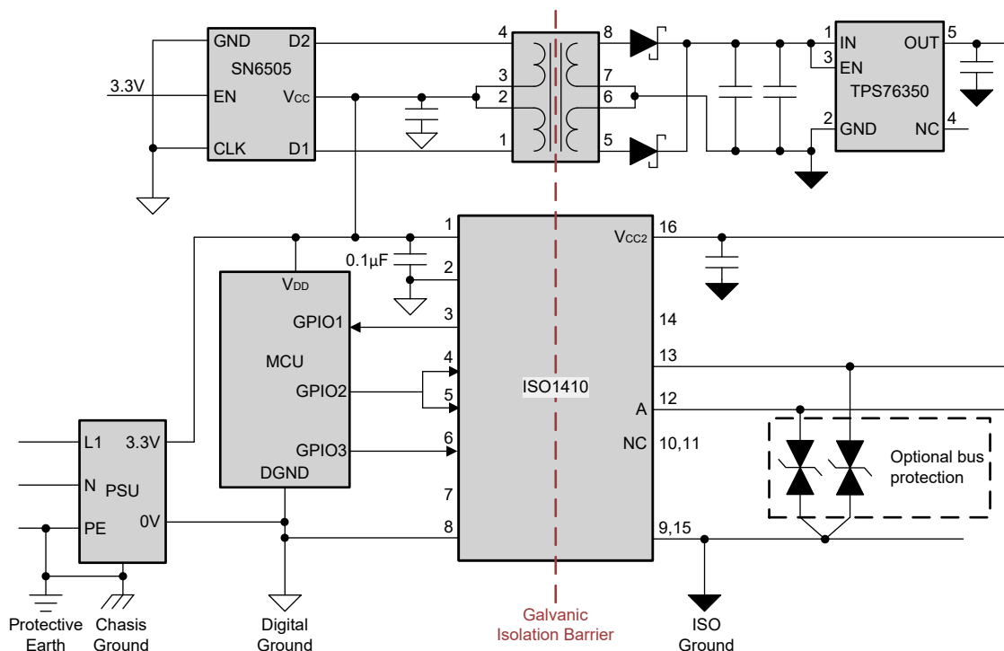
Figure 9-3. Application Circuit of ISO1410
