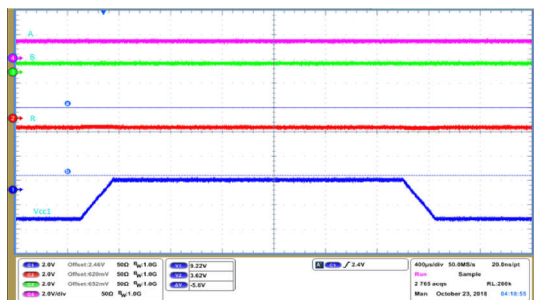
Figure 6-33. V_{CC1} Power Up/Power Down - Glitch Free Behavior
