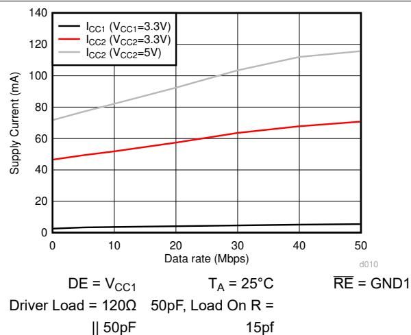
Figure 6-10. ISO145x Supply Current Vs Data Rate- 120Ω||50pF Load
