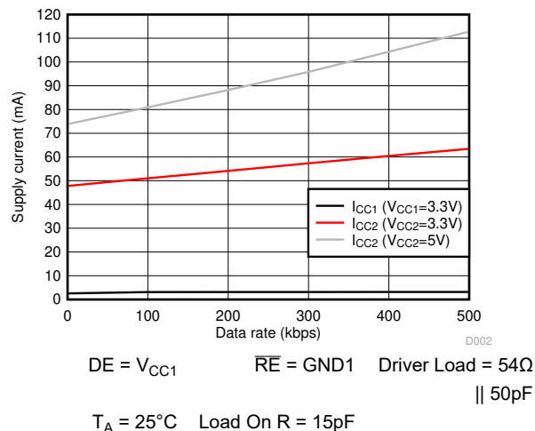
Figure 6-4. ISO141x Supply Current Vs Data Rate- With 54\Omega || 50\text{pF} Load
