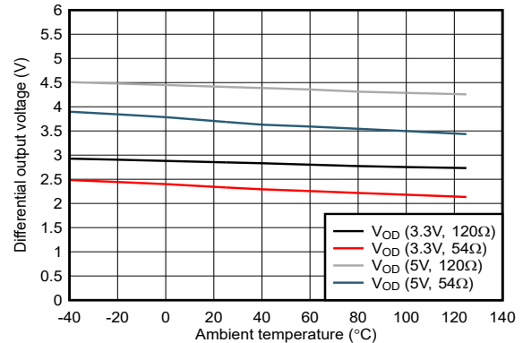
Figure 6-14. Driver Differential Output Voltage Vs Temperature
