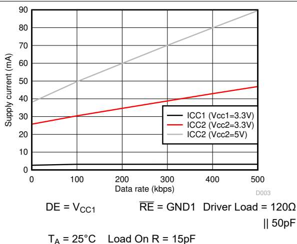
Figure 6-5. ISO141x Supply Current Vs Data Rate- With 120\Omega || 50\text{pF} Load
