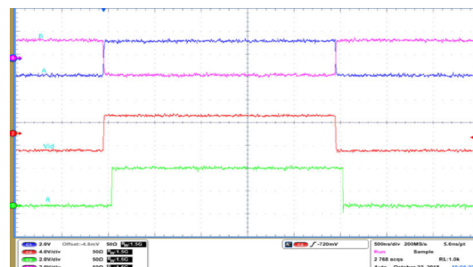
Figure 6-30. ISO143x Driver Propagation Delay
