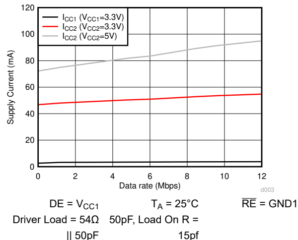
Figure 6-8. ISO143x Supply Current Vs Data Rate- 54Ω||50pF Load
