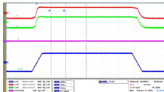
Figure 6-34. V_{CC2} Power Up/Power Down - Glitch Free Behavior
