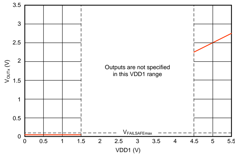
Figure 46. ISO224 Failsafe Output Behavior With V_{\text{IN}} = 0 V
