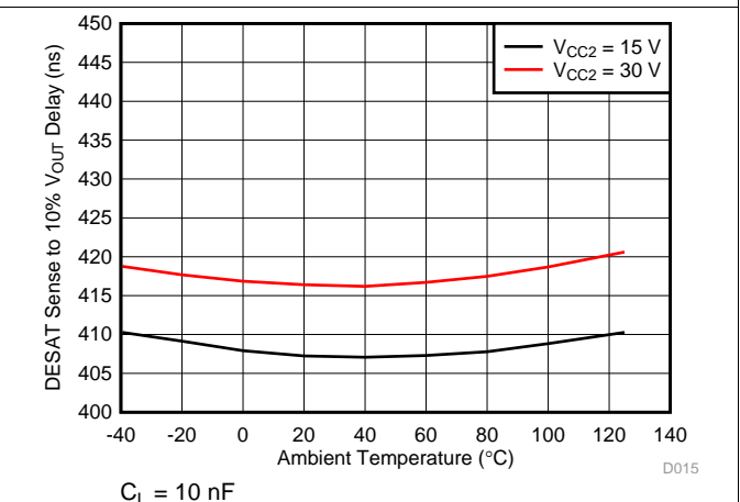
Figure 30. DESAT Sense to V_{OUT} 10% Delay vs Temperature
