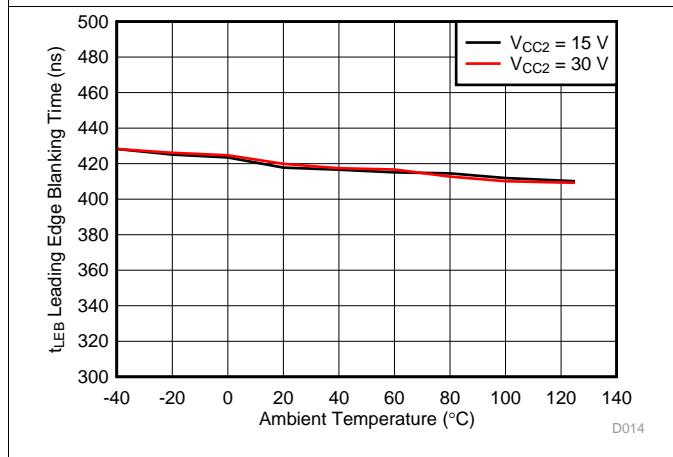
Figure 29. Leading Edge Blanking Time With Temperature
