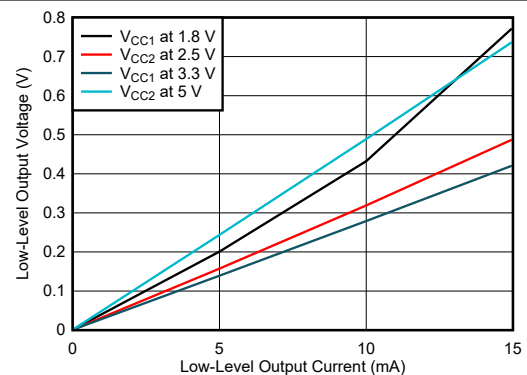
Figure 5-14. Low-Level Output Voltage vs Low-Level Output Current
