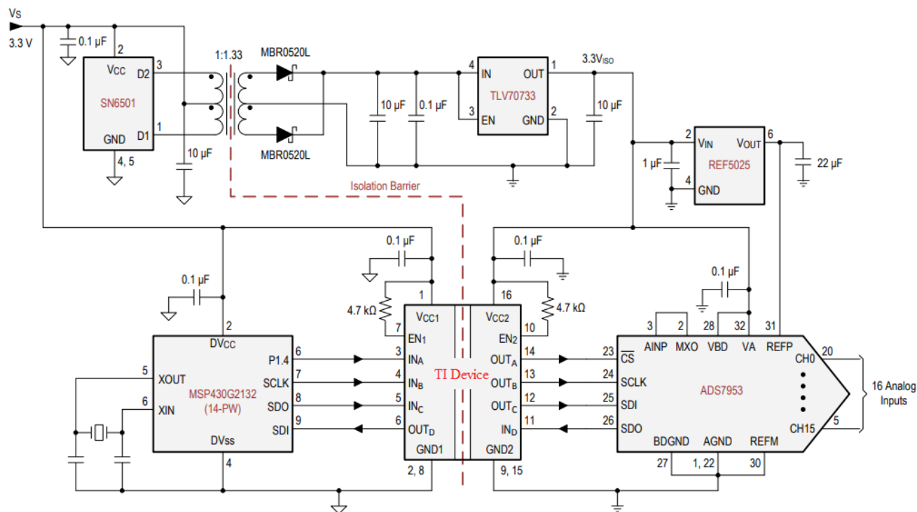
Figure 8-6. Isolated SPI for an Analog Input Module With 16 Inputs
