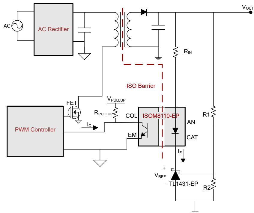
Figure 8-1. Typical Isolated Power Supply Application Using ISOM8110-EP
