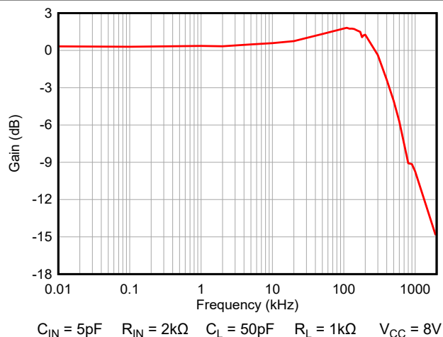
Figure 8-3. Bandwidth at R_L = 1\text{k}\Omega
