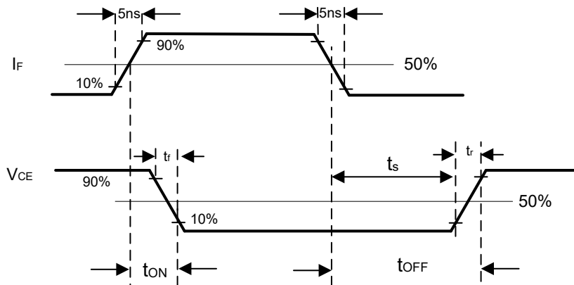
Figure 7-3. ISOM811x-Q1 Switching Timing Waveforms
