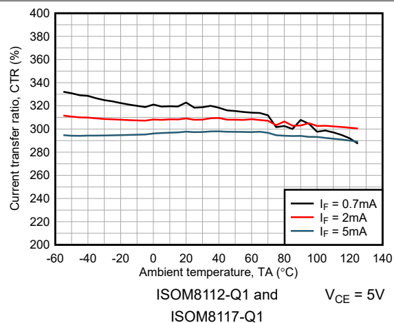
Figure 6-24. Current Transfer Ratio vs Ambient Temperature
