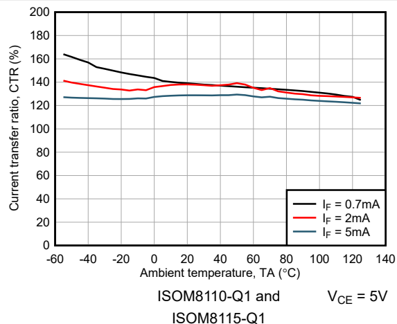
Figure 6-22. Current Transfer Ratio vs Ambient Temperature
