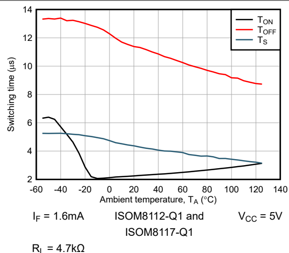
Figure 6-32. Switching Time vs Ambient Temperature
