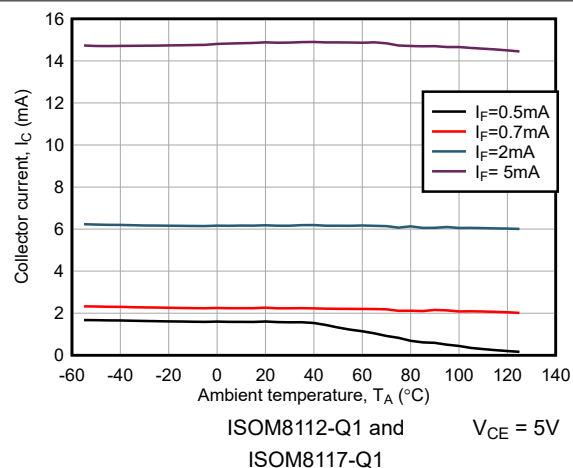
Figure 6-20. Collector Current vs Ambient Temperature
