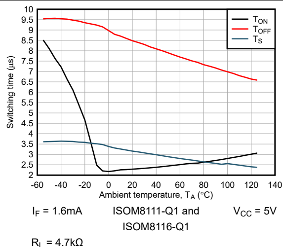
Figure 6-31. Switching Time vs Ambient Temperature
