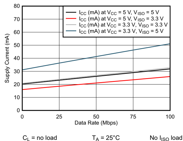
Figure 7-12. ISOW7841A-Q1 Supply Current vs Data Rate
