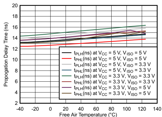
Figure 7-14. Propagation Delay Time vs Free-Air Temperature
