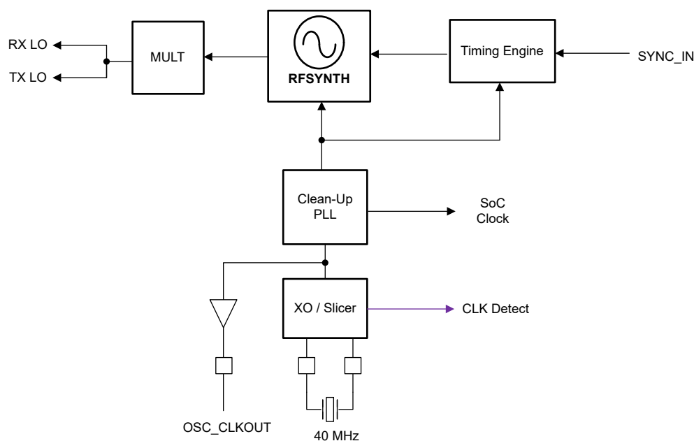
Figure 8-2. Clock Subsystem
