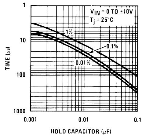
Figure 4. Acquisition Time
