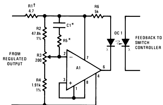
Figure 67. Light Meter
