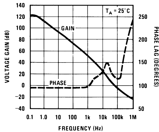
Figure 37. Frequency Response
