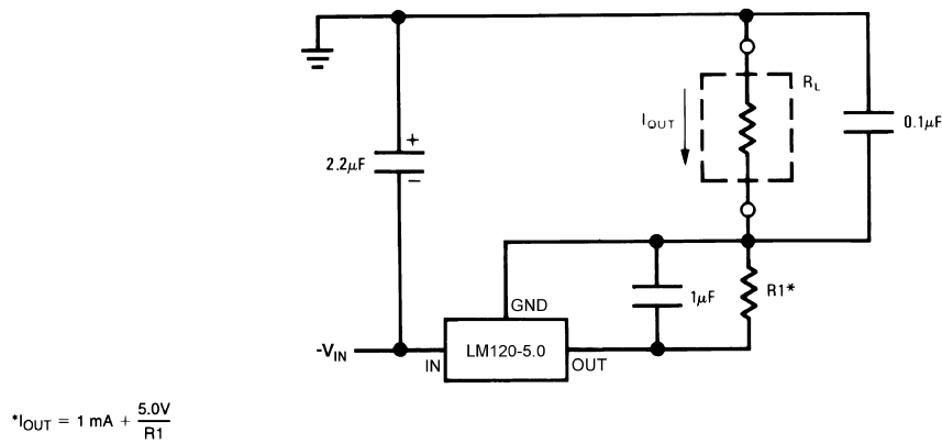
Figure 18. Current Source
