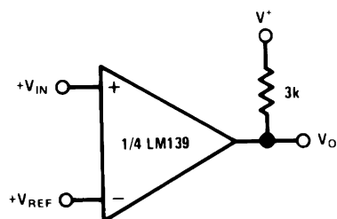
Figure 6-16. Basic Comparator
