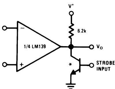
Figure 6-19. Output Strobing
