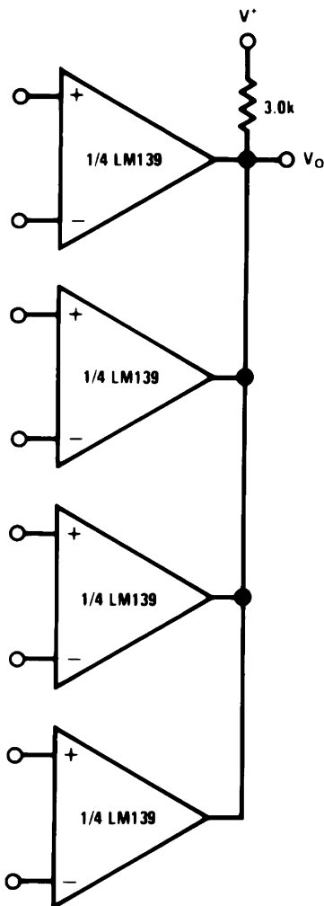
Figure 6-11. ORing the Outputs
