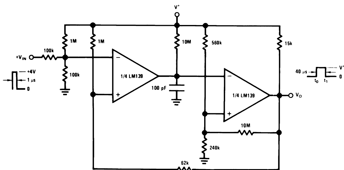
Figure 6-8. One-Shot Multivibrator With Input Lock Out
