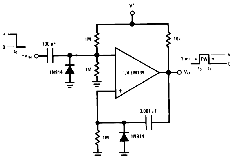
Figure 6-6. One-Shot Multivibrator
