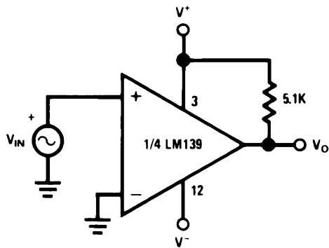
Figure 6-25. Zero Crossing Detector
