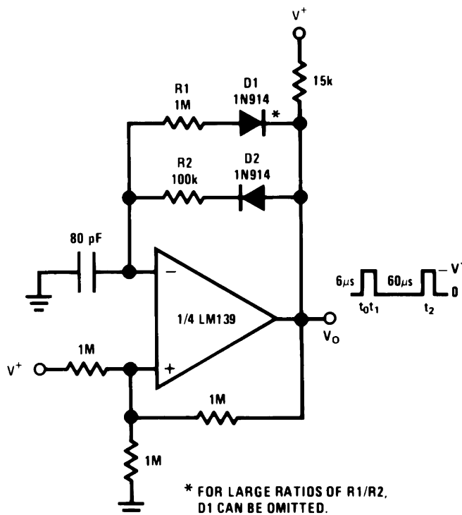
Figure 6-9. Pulse Generator
