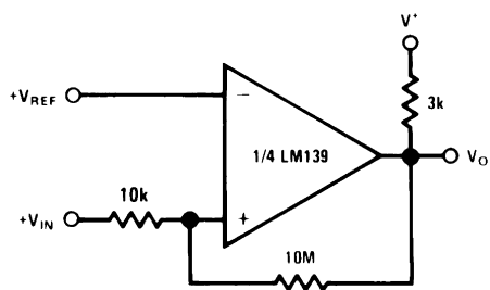
Figure 6-13. Non-Inverting Comparator With Hysteresis
