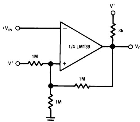
Figure 6-14. Inverting Comparator With Hysteresis
