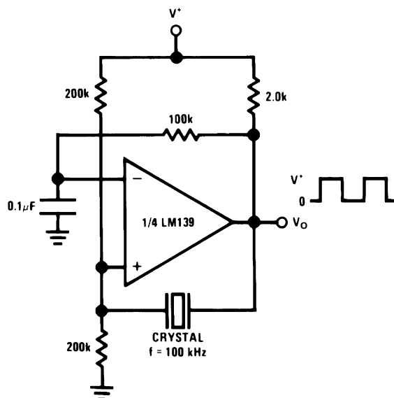
Figure 6-20. Crystal Controlled Oscillator
