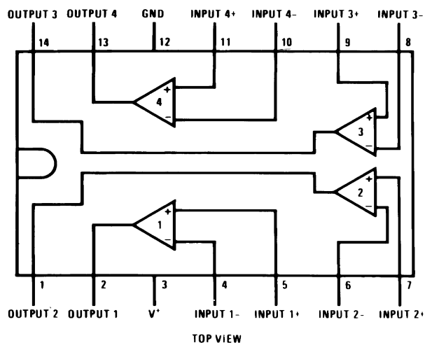
Figure 4-1. J, DYY Packages 14-Pin CDIP, SOT-23-14 Top View
