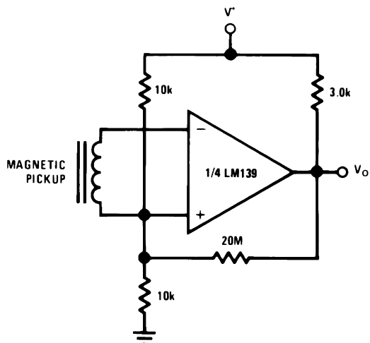
Figure 6-22. Transducer Amplifier
