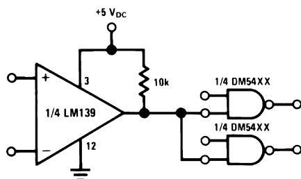
Figure 6-3. Driving TTL
