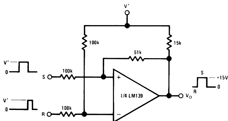
Figure 6-7. Bi-Stable Multivibrator
