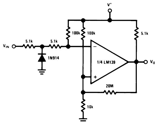
Figure 6-23. Zero Crossing Detector (Single Power Supply)
