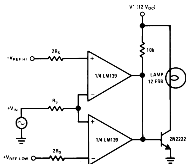
Figure 6-17. Limit Comparator
