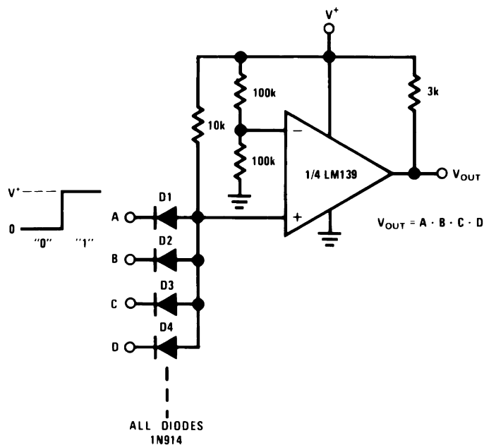
Figure 6-10. Large Fan-In AND Gate
