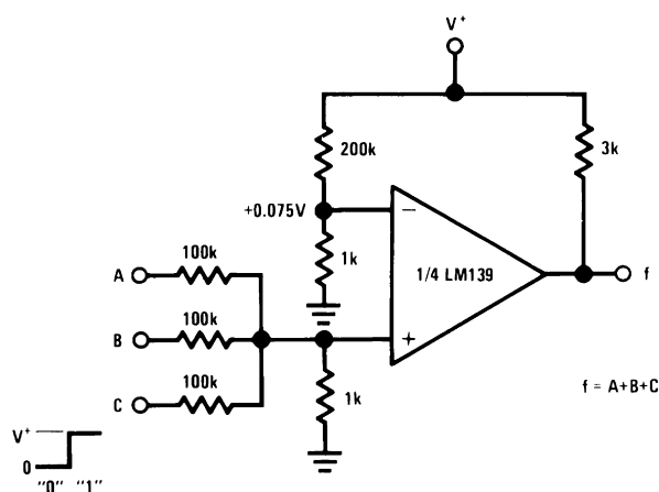
Figure 6-5. OR Gate
