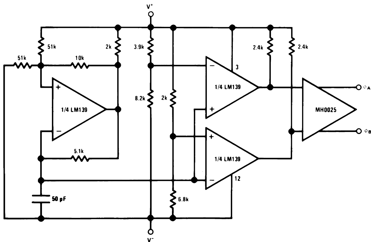
Figure 6-24. MOS Clock Driver
