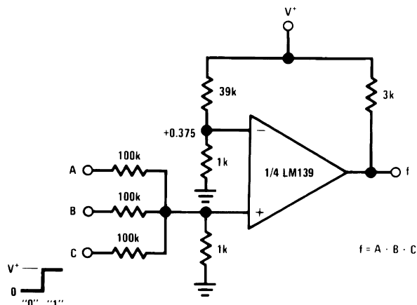
Figure 6-4. AND Gate
