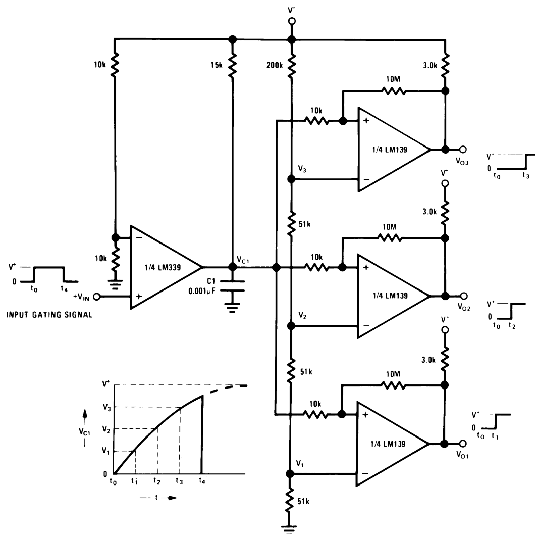
Figure 6-12. Time Delay Generator
