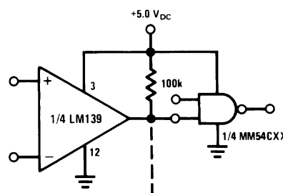
Figure 6-2. Driving CMOS
