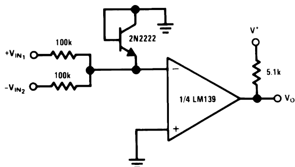
Figure 6-18. Comparing Input Voltages of Opposite Polarity
