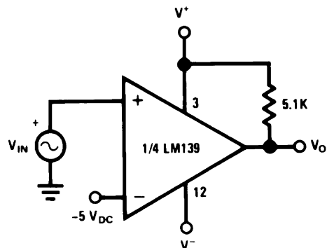
Figure 6-26. Comparator With a Negative Reference
