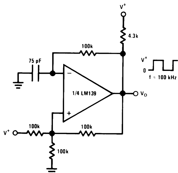
Figure 6-15. Squarewave Oscillator
