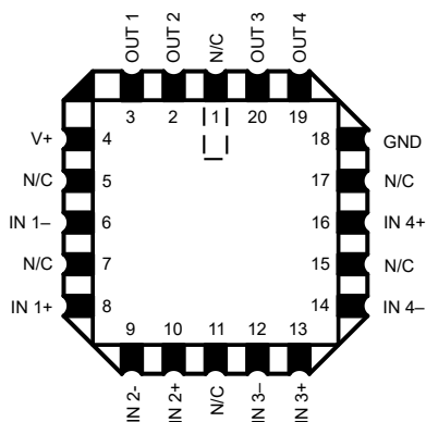
Figure 4-3. NAJ Package 20-Pad LCCC Top View
