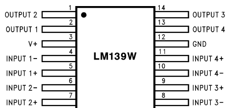
Figure 4-2. NAC, NAD Packages 14-Pin CFP (trimmed), CFP (full) Top View
