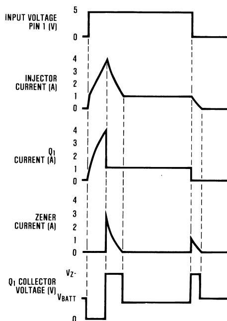
Figure 20. Circuit Waveforms
