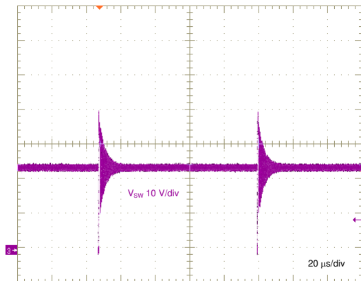
V_{IN} = 24\text{ V} I_{OUT1} = I_{OUT2} = 0\text{ A} Figure 8-23. Switch Voltage, No Load
