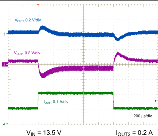
V_{IN} = 13.5\text{ V} I_{OUT2} = 0.2\text{ A} Figure 8-27. Positive Output Load Transient, 0.1 A to 0.2 A
