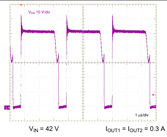
V_{IN} = 42\text{ V} I_{OUT1} = I_{OUT2} = 0.3\text{ A} Figure 8-26. Switch Voltage, Full Load
