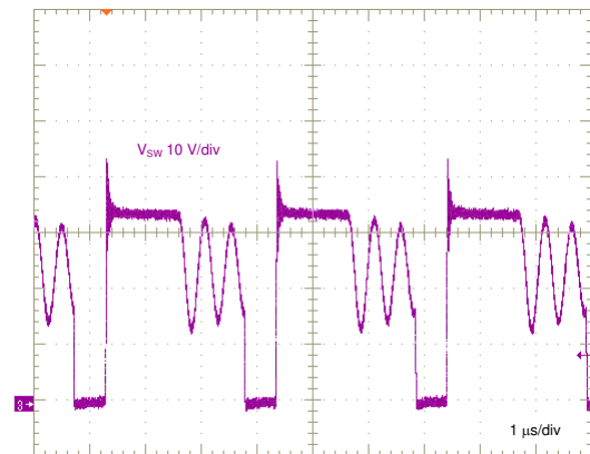
V_{IN} = 24\text{ V} I_{OUT1} = I_{OUT2} = 0.1\text{ A} Figure 8-24. Switch Voltage, Medium Load
