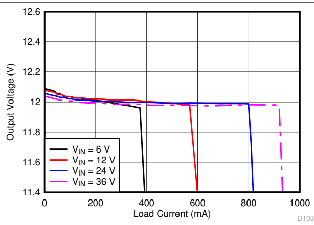
Figure 6-2. Output Voltage versus Load
