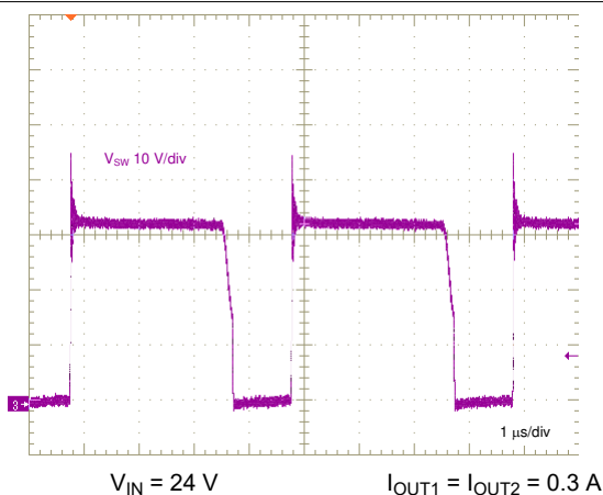
V_{IN} = 24\text{ V} I_{OUT1} = I_{OUT2} = 0.3\text{ A} Figure 8-25. Switch Voltage, Full Load
