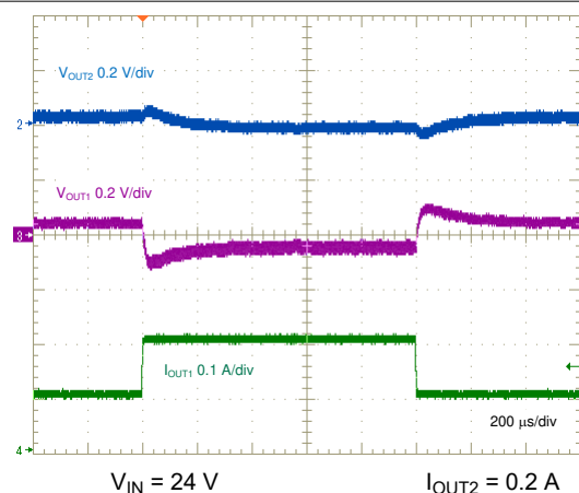
V_{IN} = 24\text{ V} I_{OUT2} = 0.2\text{ A} Figure 8-28. Positive Output Load Transient, 0.1 A to 0.2 A
