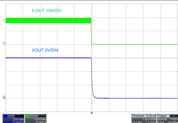
Figure 10-6. Shutdown, EN OFF, V_{SUPPLY} = 12V , I_{LOAD} = 18A Resistive Load
