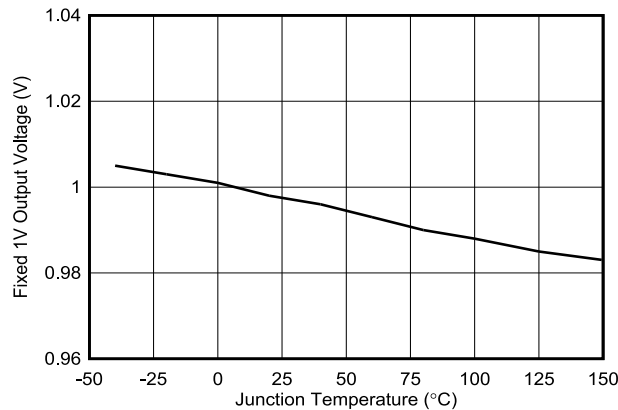
Figure 6-5. Fixed Output Voltage vs Temperature, V_{OUT} = 1V
