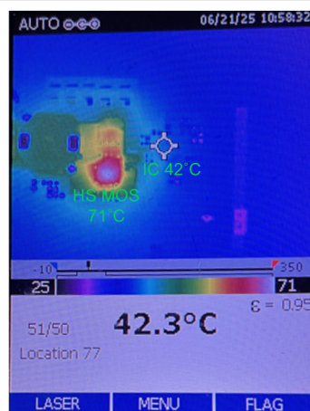
Figure 10-10. V_{SUPPLY} = 16V , I_{LOAD} = 20A , T_A = 25^\circ C , No Airflow
