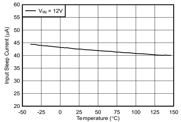
Figure 6-4. Input Sleep Current vs Temperature, V_{OUT} = 5V
