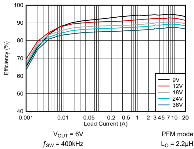
Figure 6-1. Efficiency PFM Mode
