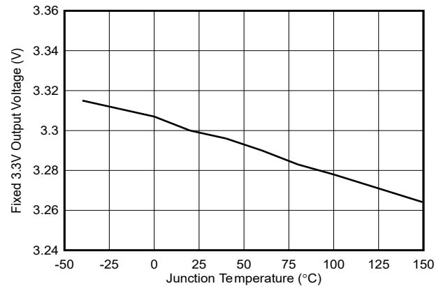
Figure 6-6. Fixed Output Voltage vs Temperature, V_{OUT} = 3.3V
