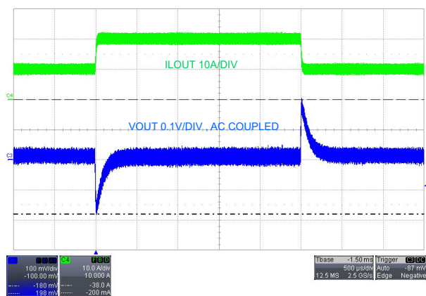
Figure 10-8. Load Transient Response, V_{SUPPLY} = 12V , FPWM, 10A to 20A
