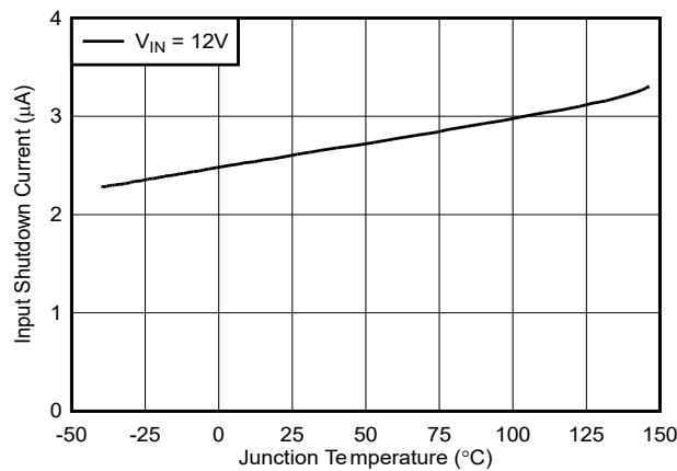
Figure 6-3. Input Shutdown Current vs Temperature
