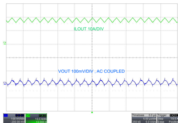
Figure 10-7. Output Ripple, V_{SUPPLY} = 12V , I_{LOAD} = 18A
