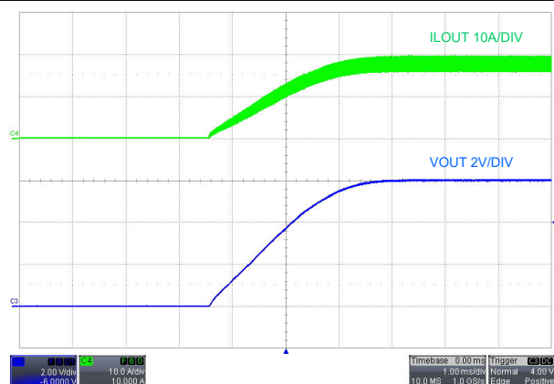
Figure 10-5. Start-Up, EN ON, V_{SUPPLY} = 12V , I_{LOAD} = 18A Resistive Load
