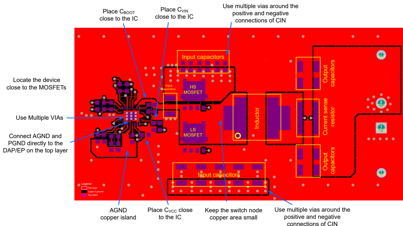
Figure 10-12. PCB Top Layer
