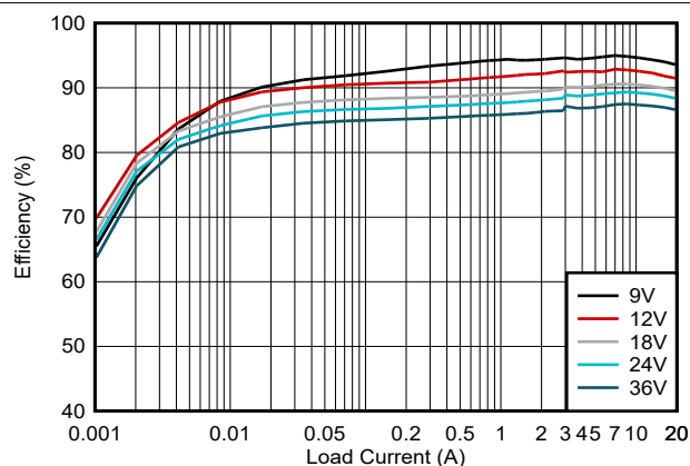
Figure 10-9. PFM Mode Efficiency, Log Scale
