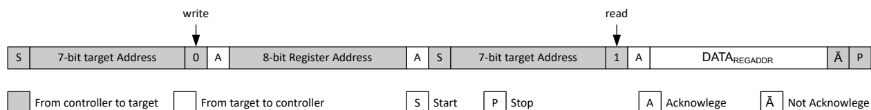
Figure 8-4. Single READ From a Defined Register Address
