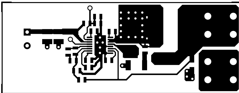
Figure 7-11. Component Side
