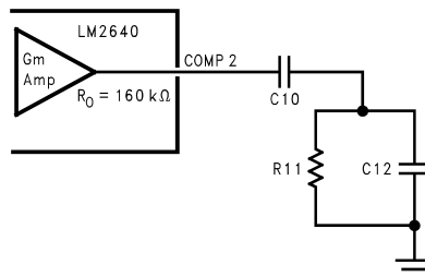
Figure 26. Typical Compensation Network
