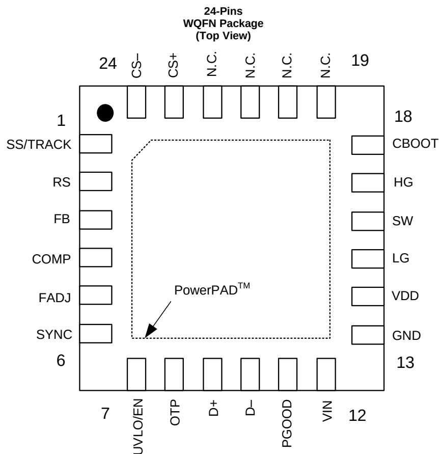
Pin Functions
