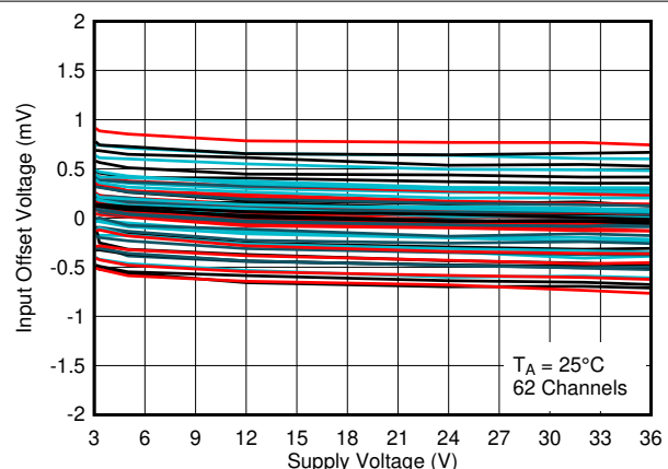
Figure 2-12. Input Offset Voltage vs. Supply Voltage at 25°C
