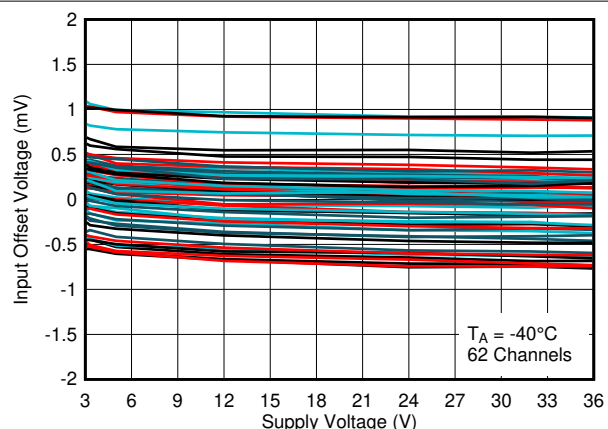
Figure 2-11. Input Offset Voltage vs. Supply Voltage at -40°C
