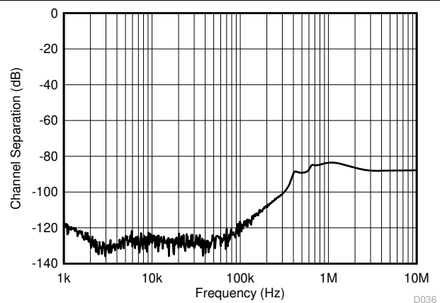
Figure 6-29. Channel Separation
